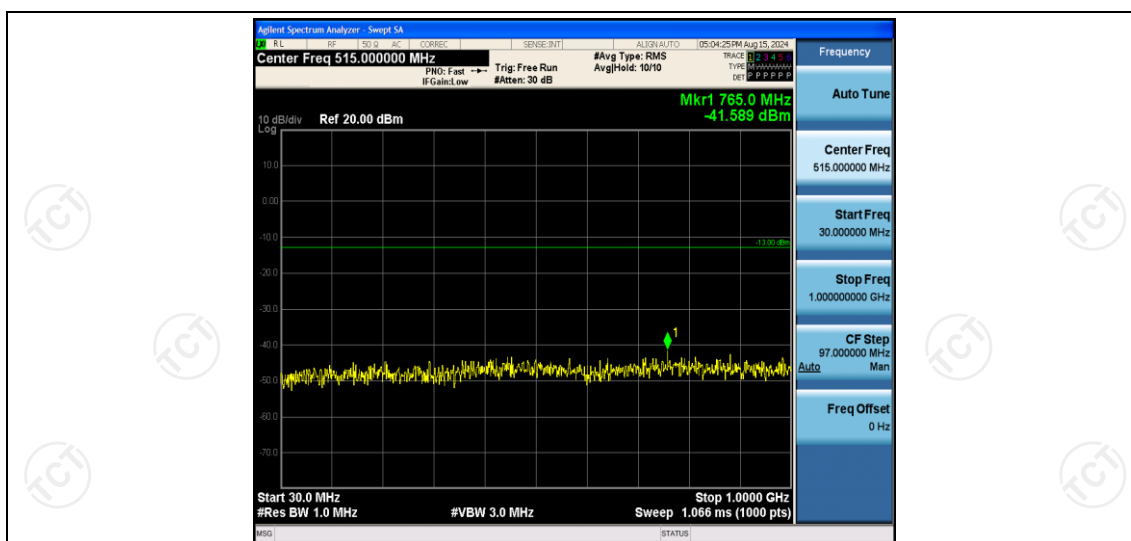
Band66-1.4MHz-QPSK-131979-1RB#0-Range1:30~1000MHz
