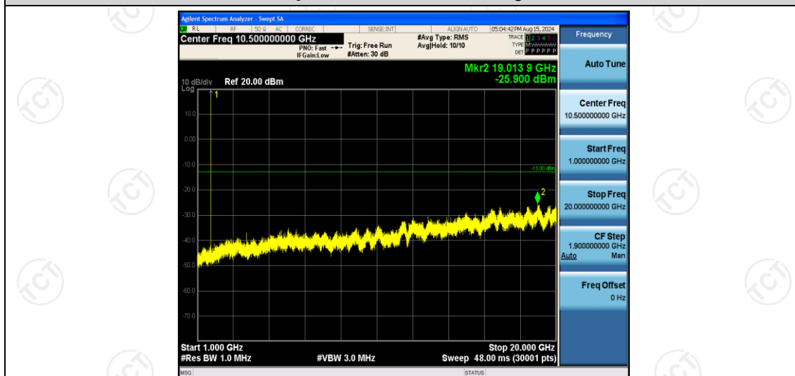
Band66-1.4MHz-QPSK-131979-1RB#0-Range2:1000~20000MHz
