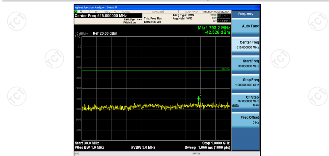
Band66-1.4MHz-QPSK-132322-1RB#0-Range1:30~1000MHz
