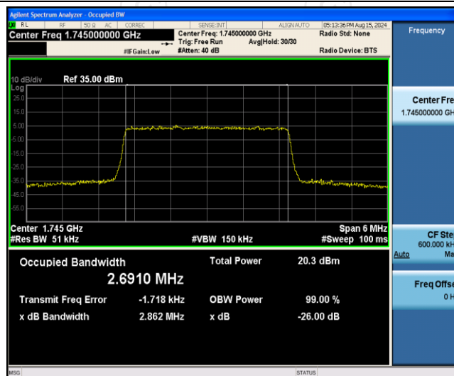
Band66-1.745GHz-16QAM-132665-6RB#0
