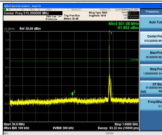
Band13-5MHz-16QAM-23205-1RB#0-Range1:30~1000MHz
