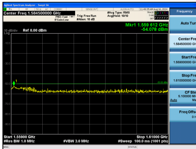
Band13-5MHz-QPSK-23230-1RB#0-Range5:1559~1610MHz
