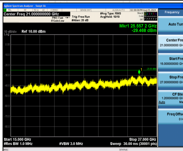
Band7-5MHz-QPSK-21100-1RB#0-Range3:15000~27000MHz
