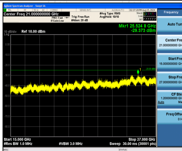
Band7-5MHz-16QAM-20775-1RB#0-Range3:15000~27000MHz
