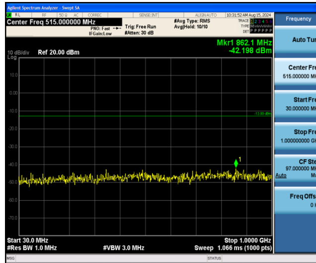
Band2-3MHz-16QAM-19185-1RB#0-Range1:30~1000MHz
