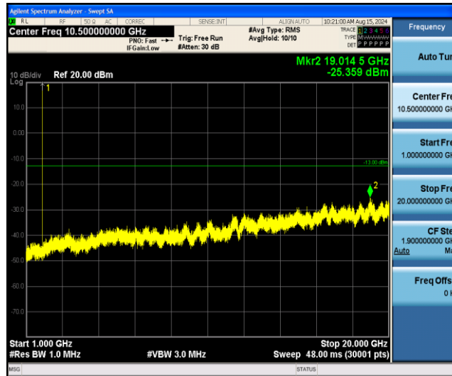
Band2-1.4MHz-QPSK-18607-1RB#0-Range2:1000~20000MHz
