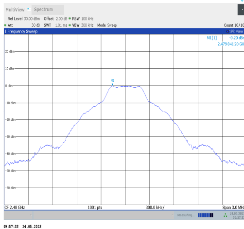
BLE_1M-Ant0-2480-0~Reference
