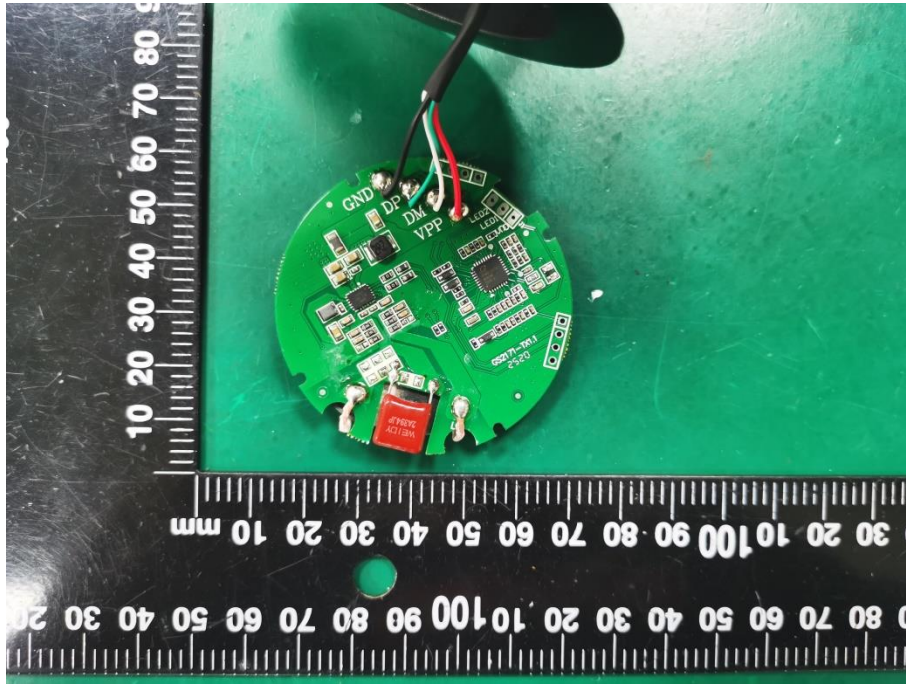
Internal Photo FCC ID: 2A68H-YY901
