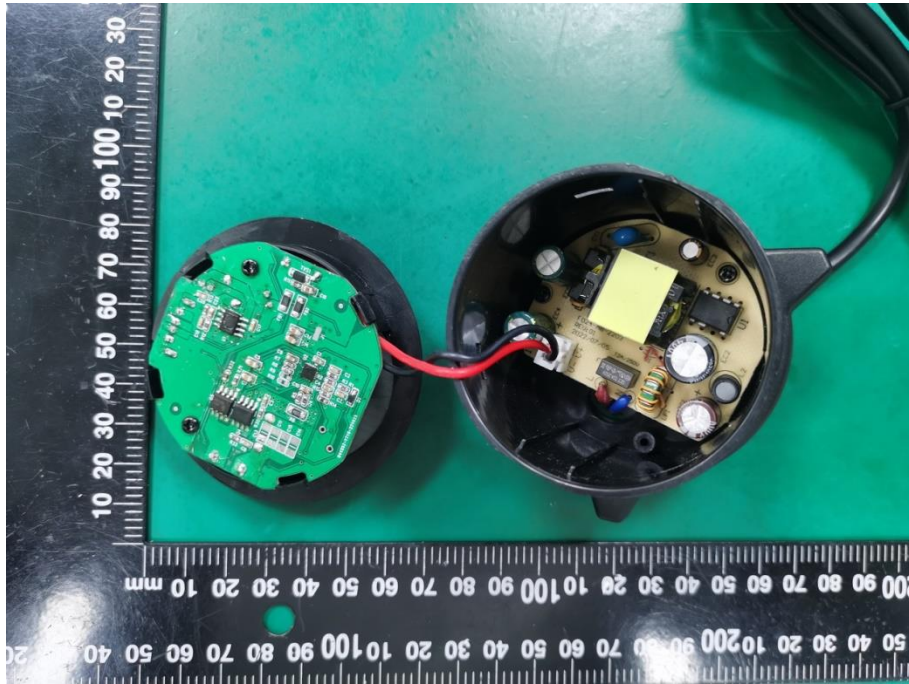
Internal Photo FCC ID: 2A68H-YY185
