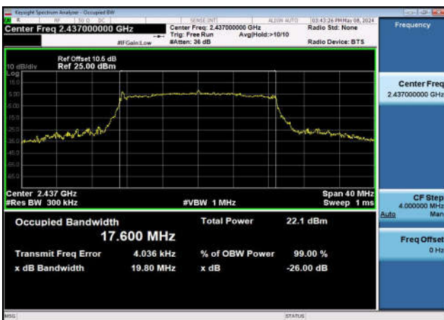
99% Bandwidth-802.11g,2437MHz,Ant0
