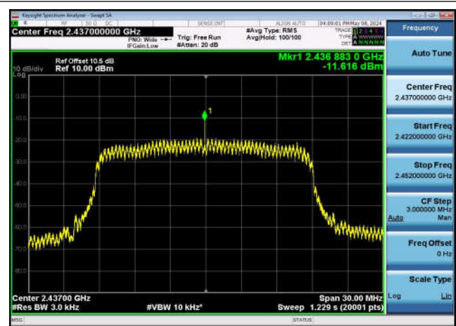
Power spectral density-802.11n(20MHz) ,2437MHz,Ant0
