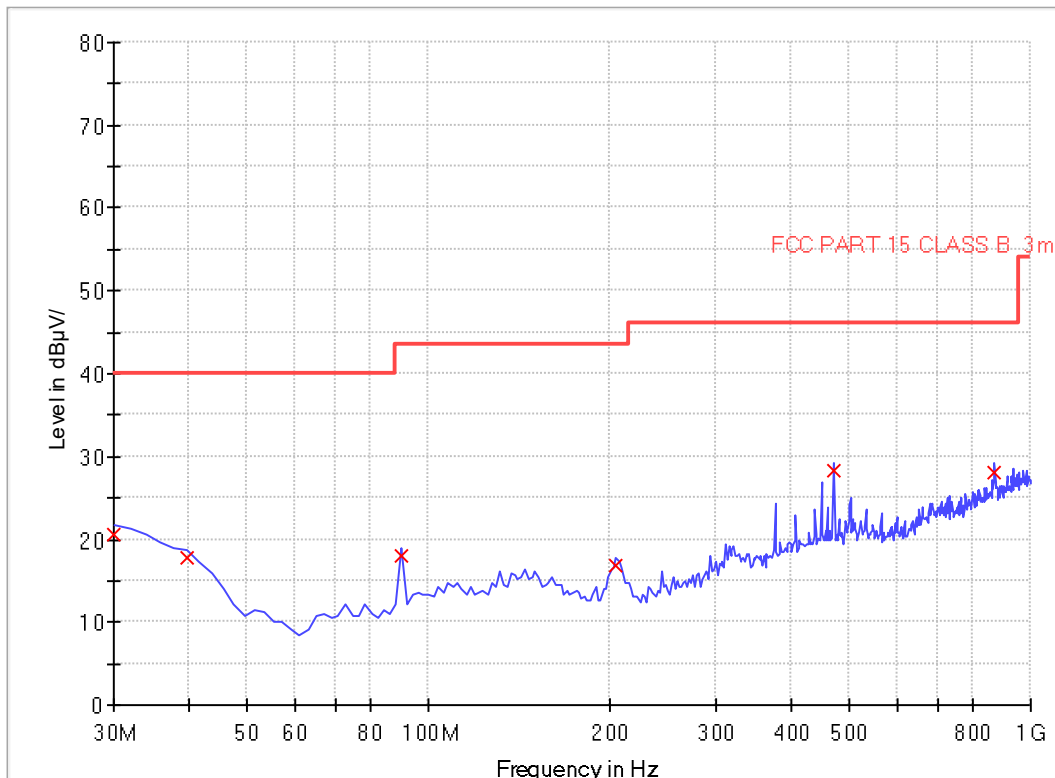
(Plot C: Test Antenna Vertical 30M - 1G)
