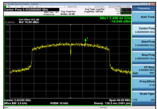
Power spectral density-802.11ax(HE40) ,2452MHz,Ant0
