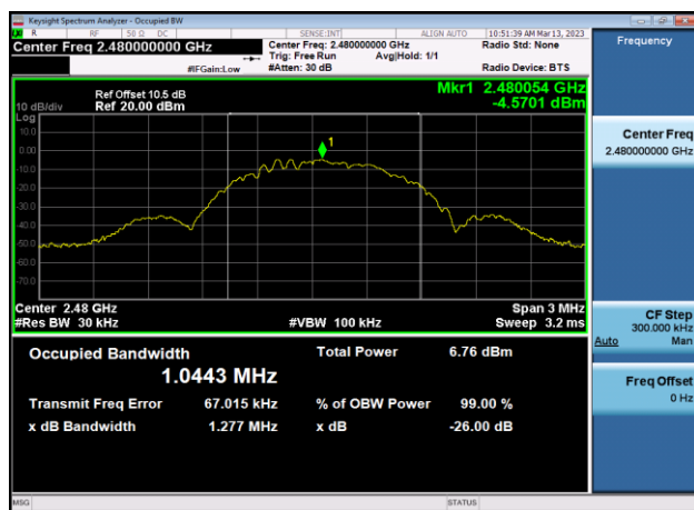
99% Bandwidth: 2480MHz
