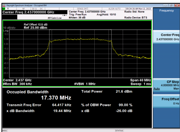
99% Bandwidth-802.11g,2437MHz,Ant0
