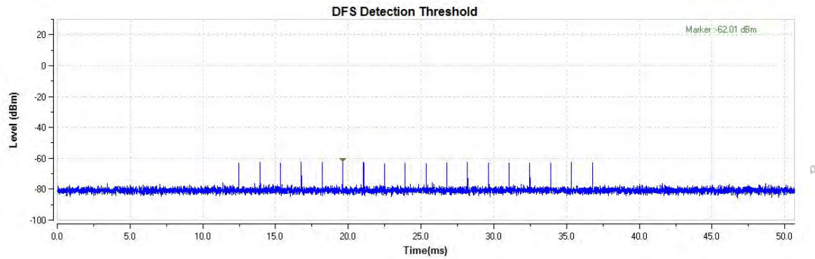
Radar Singal 0
