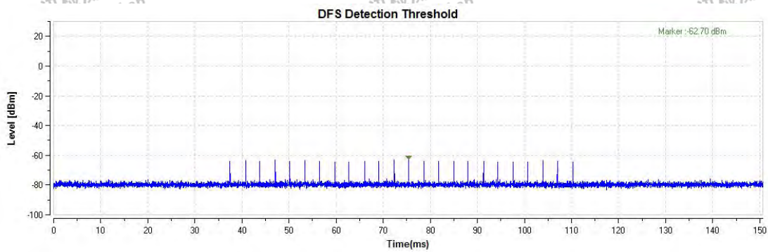
Radar Singal 5
