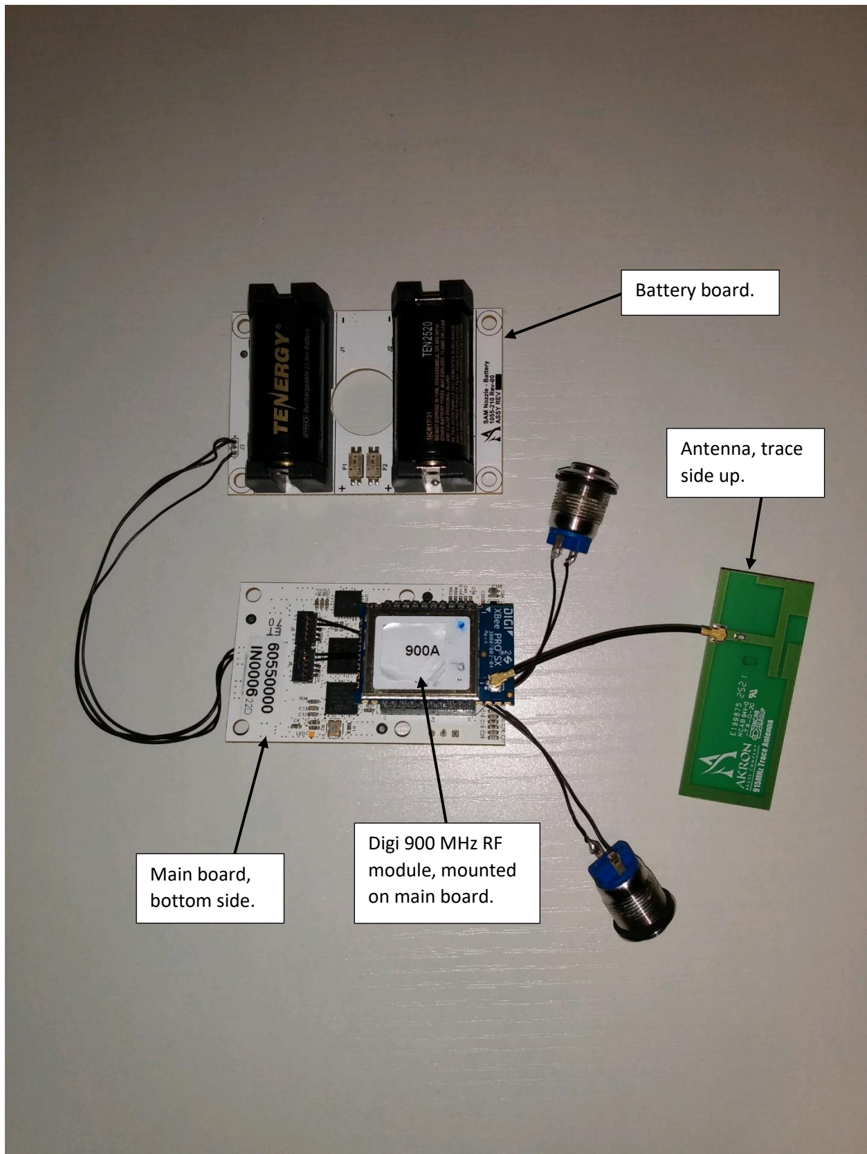
Figure 1 – 6055 SAM Smart Nozzle's electronics, separate from housing, bottom of the main board
