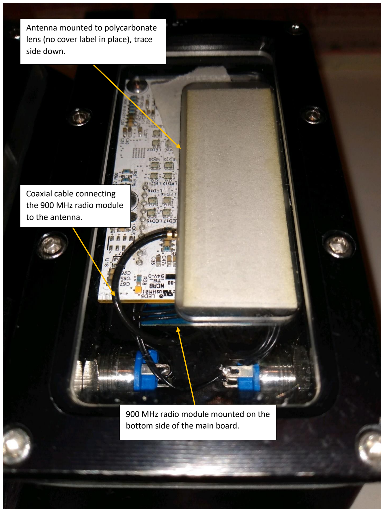
Figure 4 - Assembled 6055 SAM Smart Nozzle, top view, cover label absent
