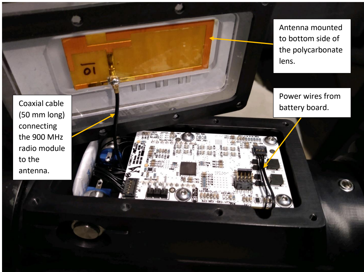
Figure 3 - Top, open view of 6055 SAM Smart Nozzle, before the polycarbonate lens is seated and fastened
