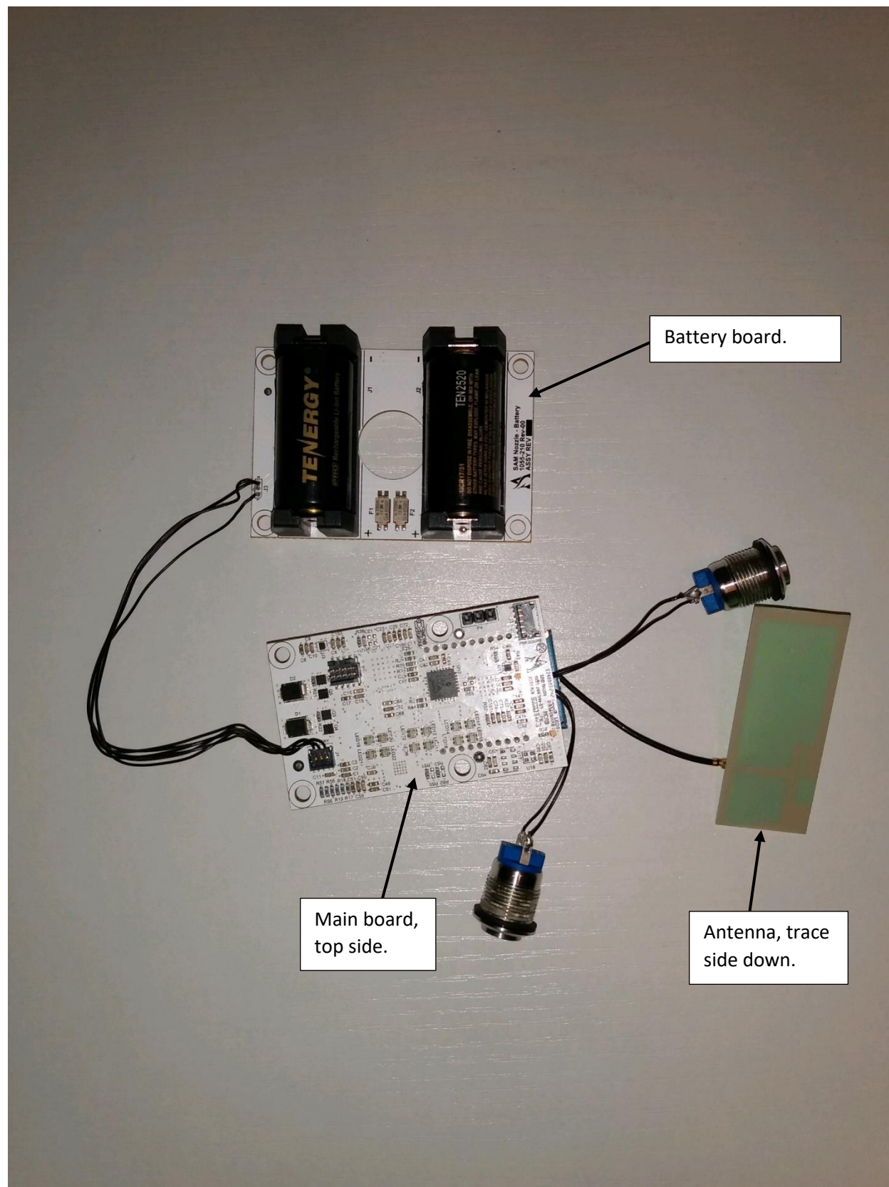
Figure 2 - 6055 SAM Smart Nozzle's electronics, separate from housing, top of the main board
