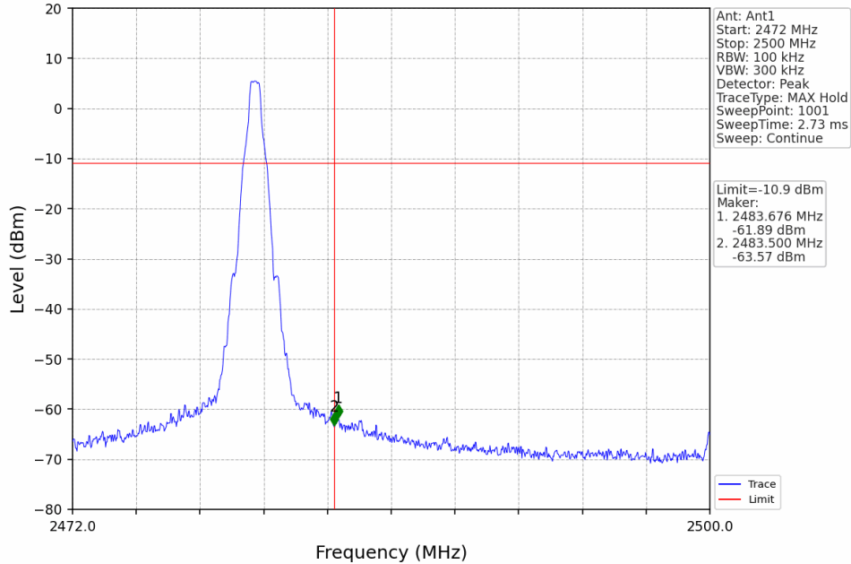
GFSK_DH5_HCH_2480MHz_Ant1_NTNV
