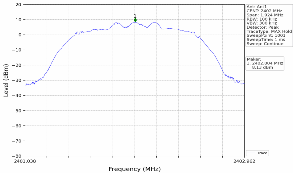
Pi/4DQPSK_2DH5_LCH_2402MHz_Ant1_NTNV
