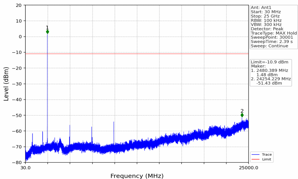
GFSK_DH5_HCH_2480MHz_Ant1_NTNV
