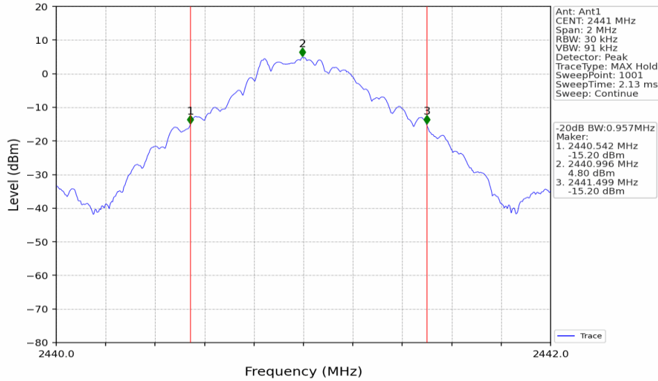
GFSK_DH5_MCH_2441MHz_Ant1_NTNV
