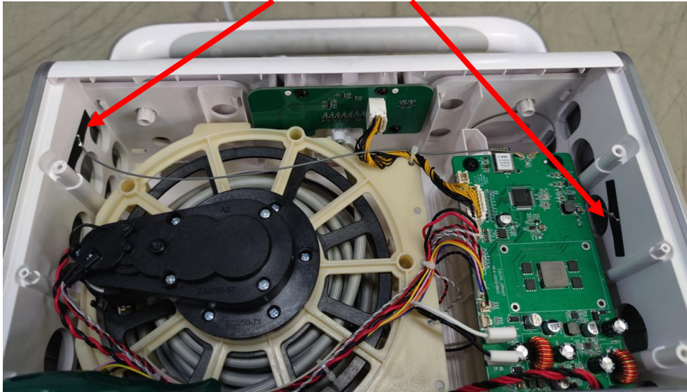
Antenna 1 Antenna 2 of station
