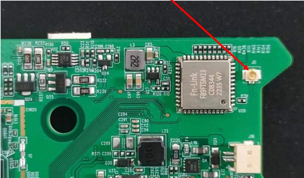
Antenna Port
