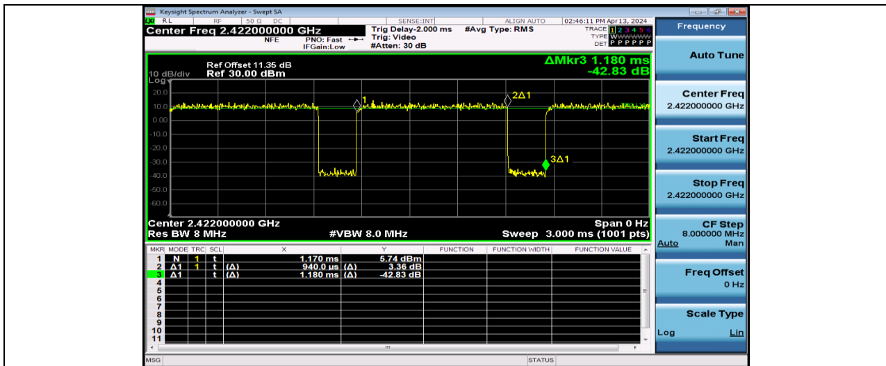
NTNV-11N40SISO-Ant1-2422
