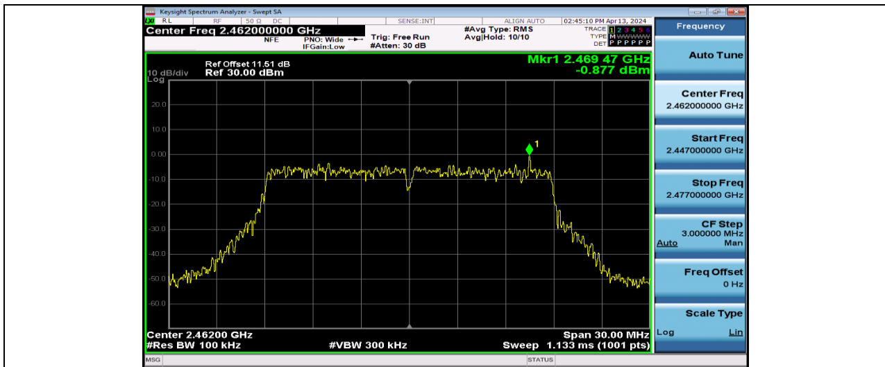
11N20SISO-Ant1-2462-0~Reference-PASS
