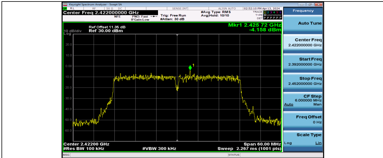
11N40SISO-Ant1-2422-0~Reference-PASS
