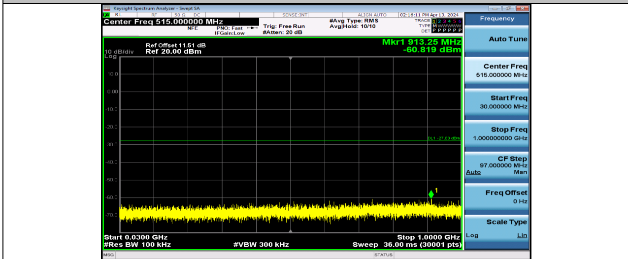
11B-Ant1-2462-30~1000-PASS
