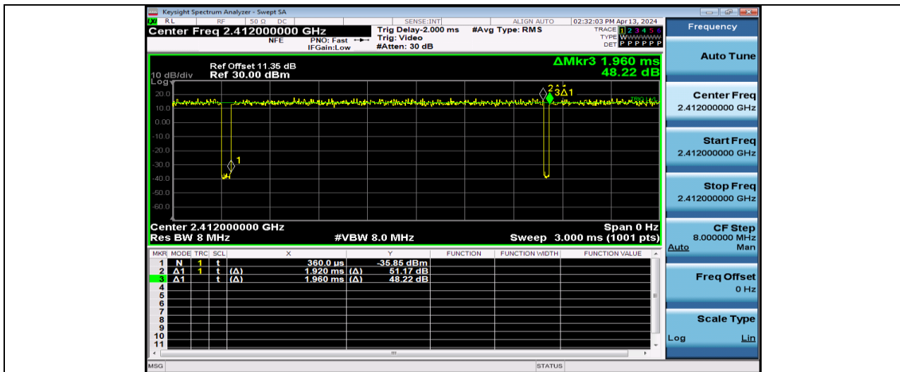
NTNV-11N20SISO-Ant1-2412
