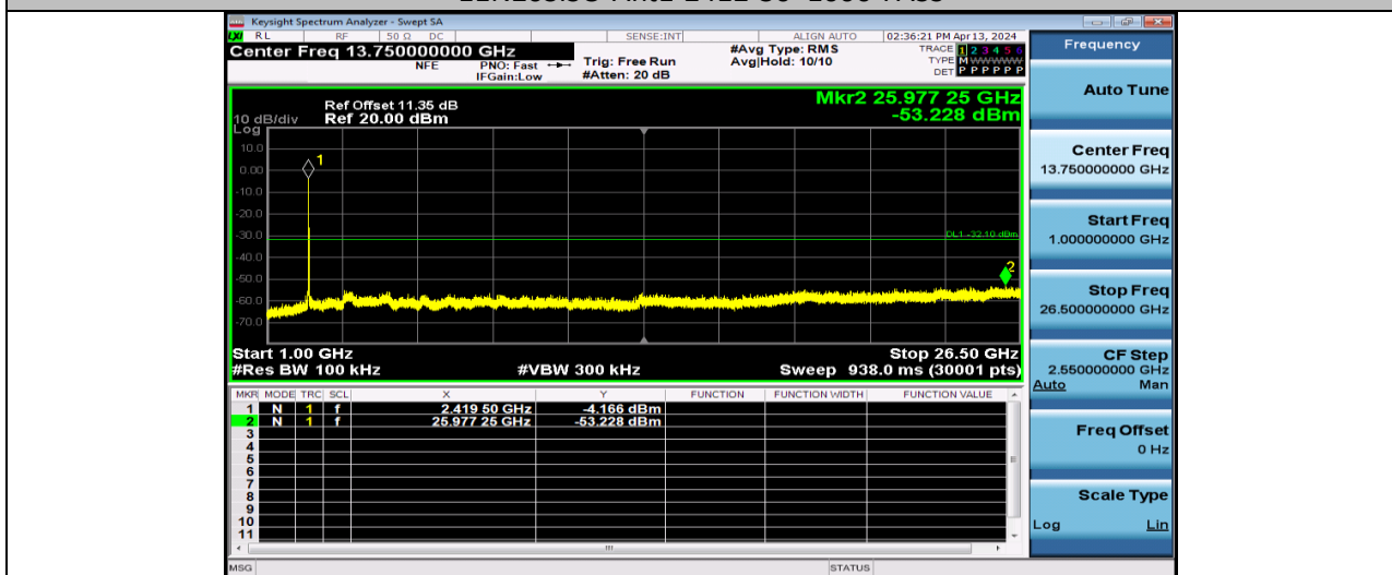
11N20SISO-Ant1-2412-1000~26500-PASS
