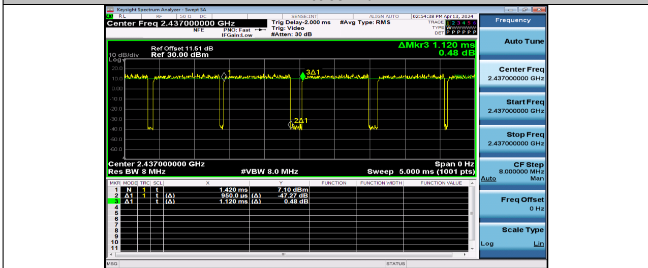
NTNV-11N40SISO-Ant1-2437
