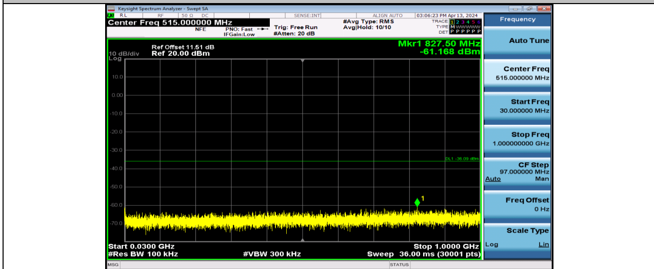
11N40SISO-Ant1-2452-30~1000-PASS
