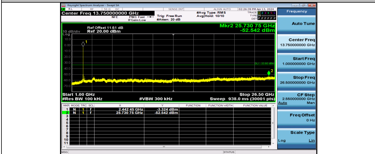
11G-Ant1-2437-1000~26500-PASS
