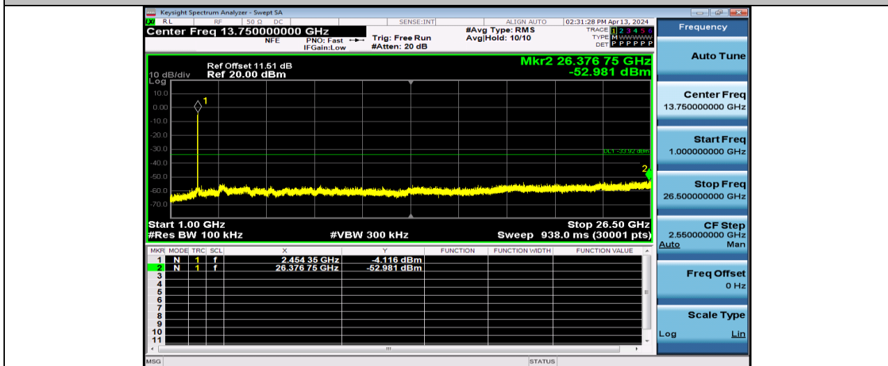
11G-Ant1-2462-1000~26500-PASS
