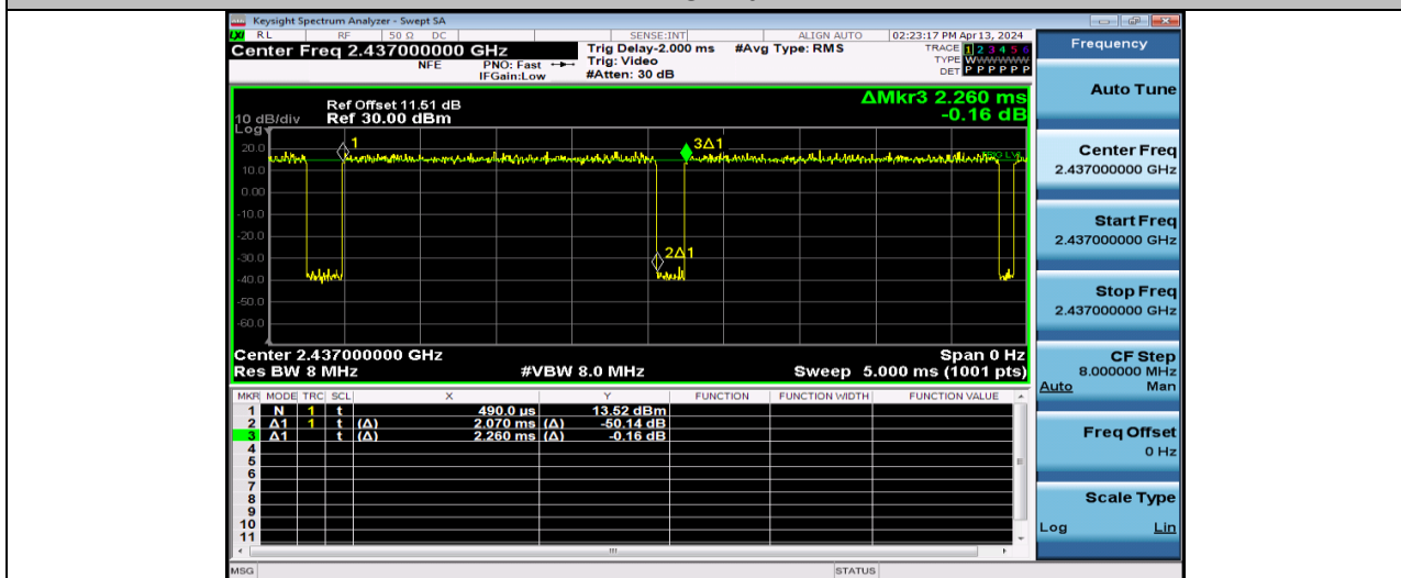
NTVN-11G-Ant1-2437
