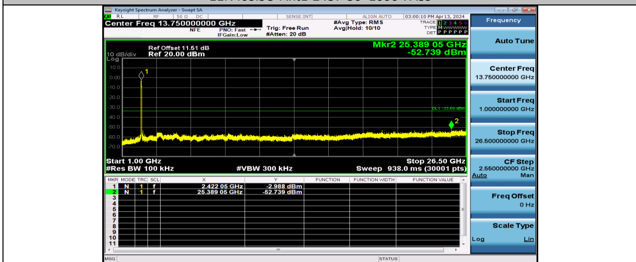
11N40SISO-Ant1-2437-1000~26500-PASS
