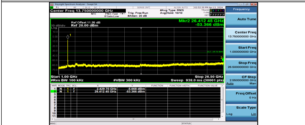
11N40SISO-Ant1-2422-1000~26500-PASS
