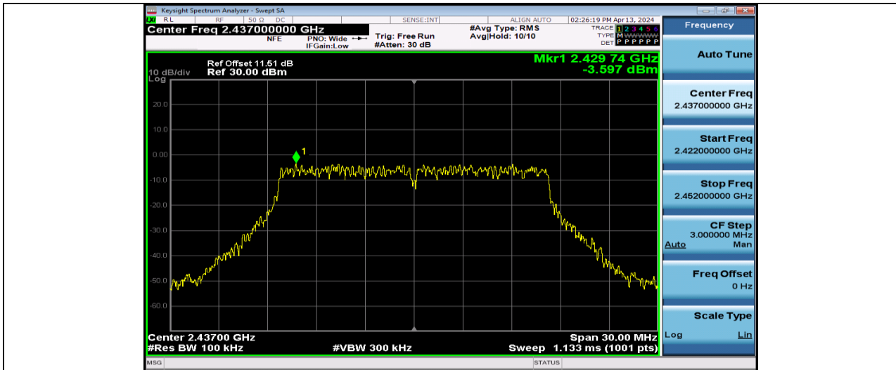
11G-Ant1-2437-0~Reference-PASS
