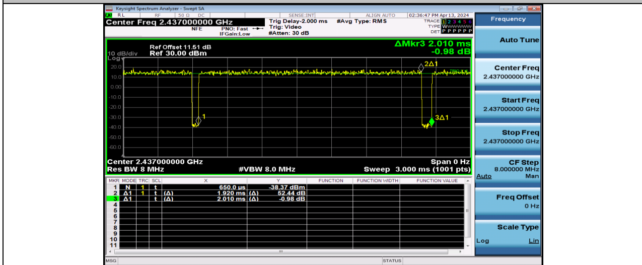
NTNV-11N20SISO-Ant1-2437
