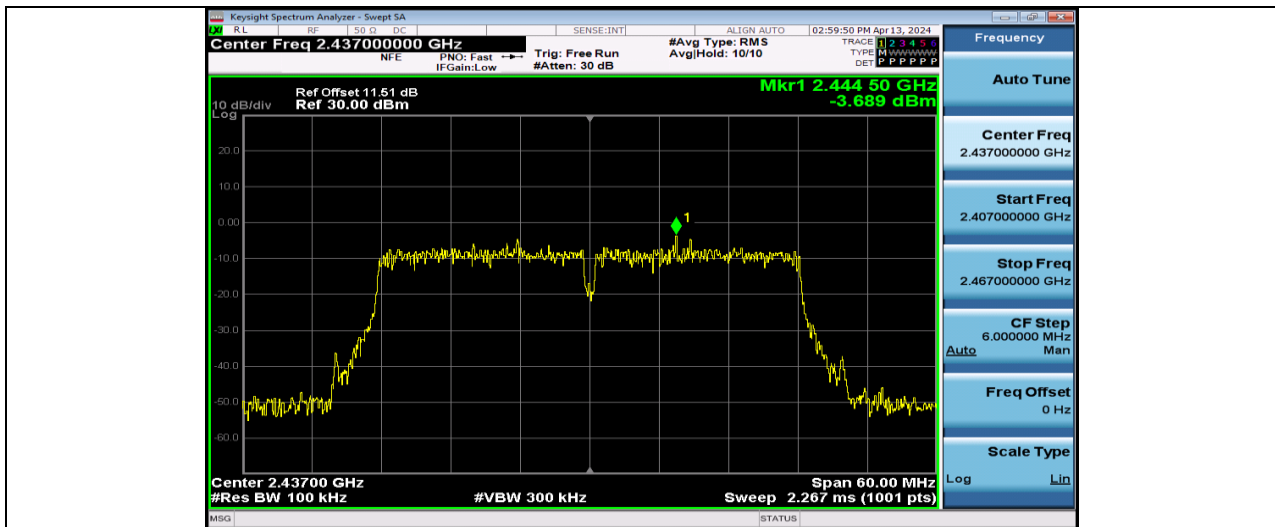
11N40SISO-Ant1-2437-0~Reference-PASS
