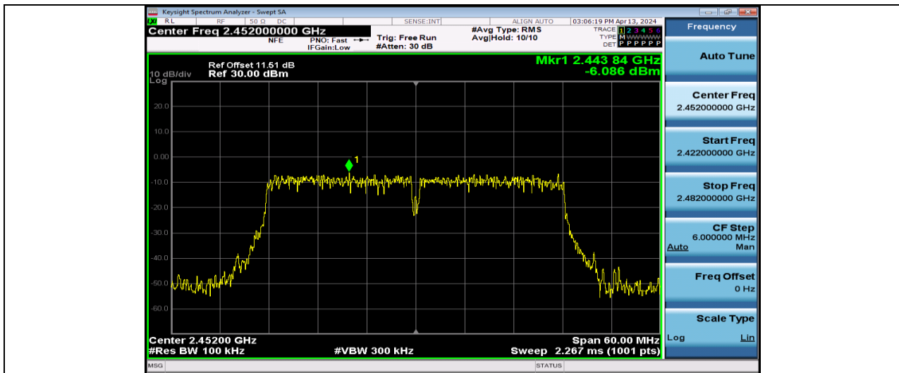
11N40SISO-Ant1-2452-0~Reference-PASS
