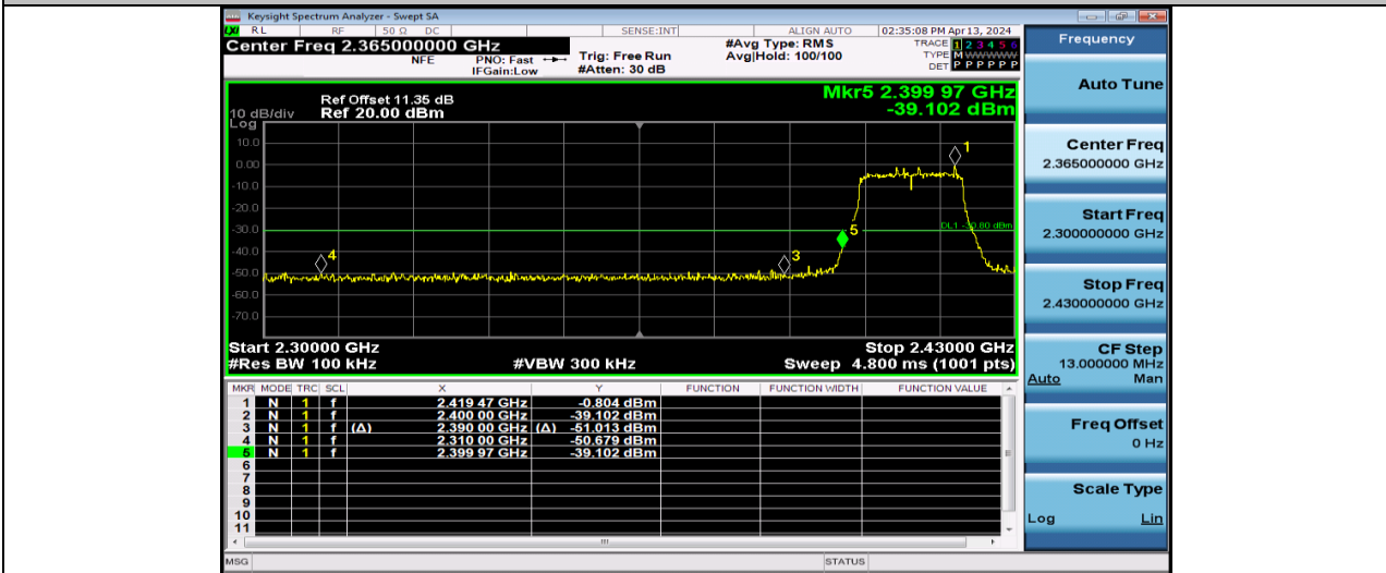
11N20SISO-Ant1-2412-PASS
