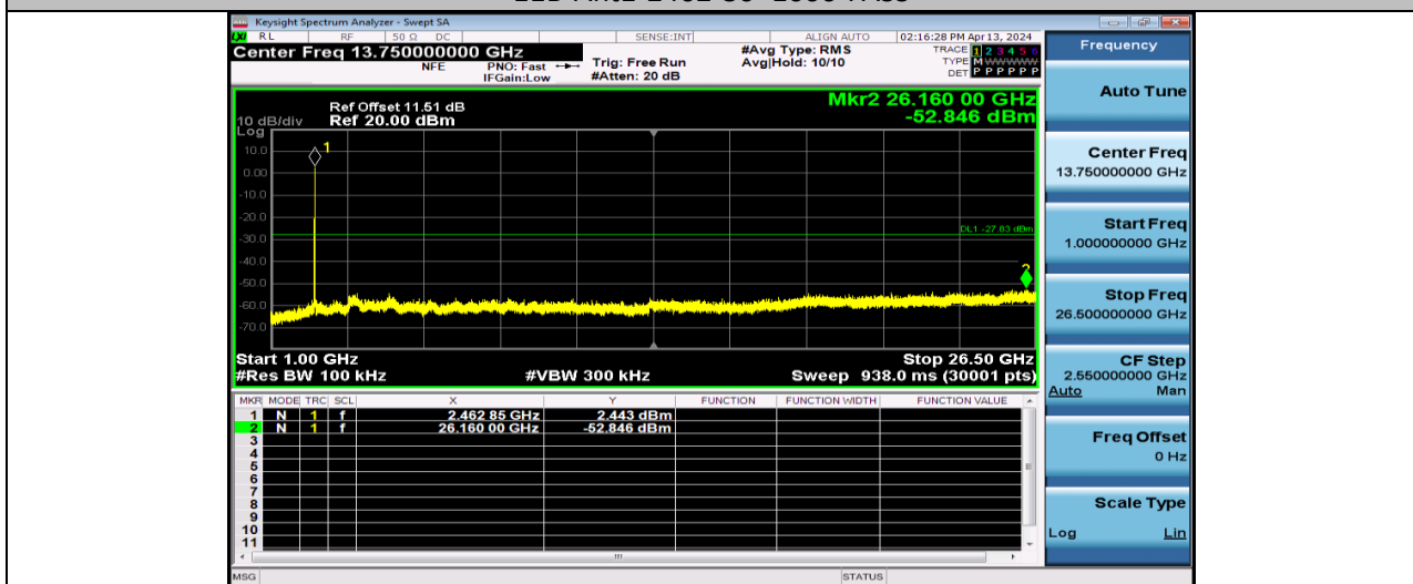
11B-Ant1-2462-1000~26500-PASS
