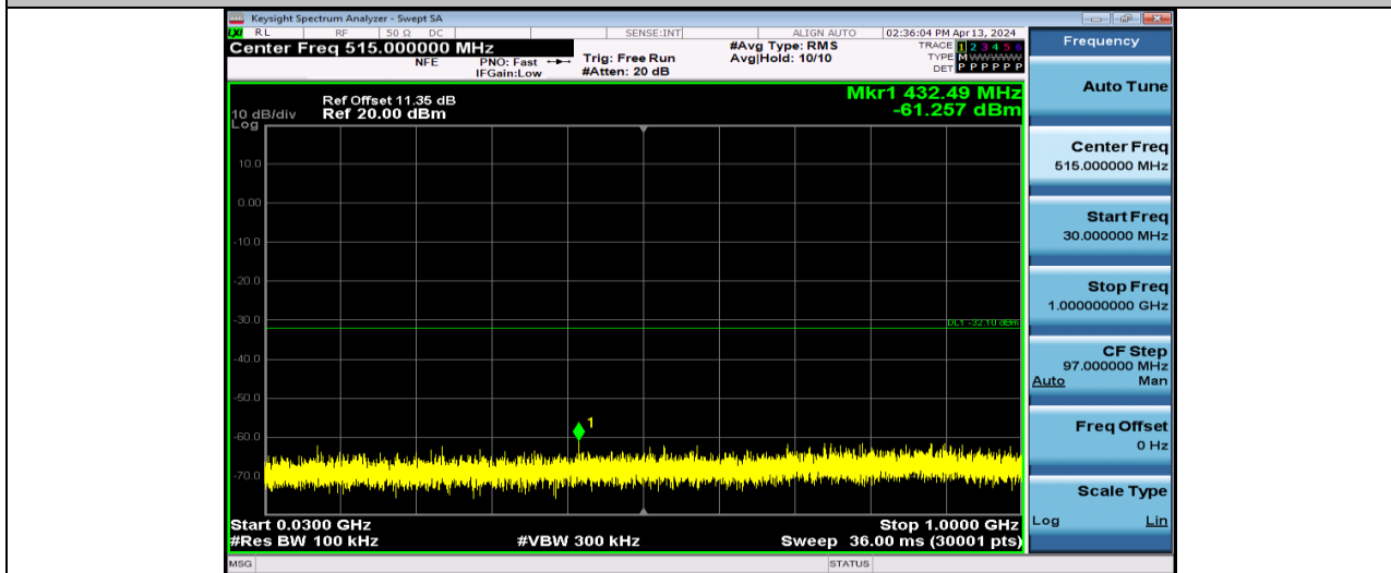
11N20SISO-Ant1-2412-30~1000-PASS
