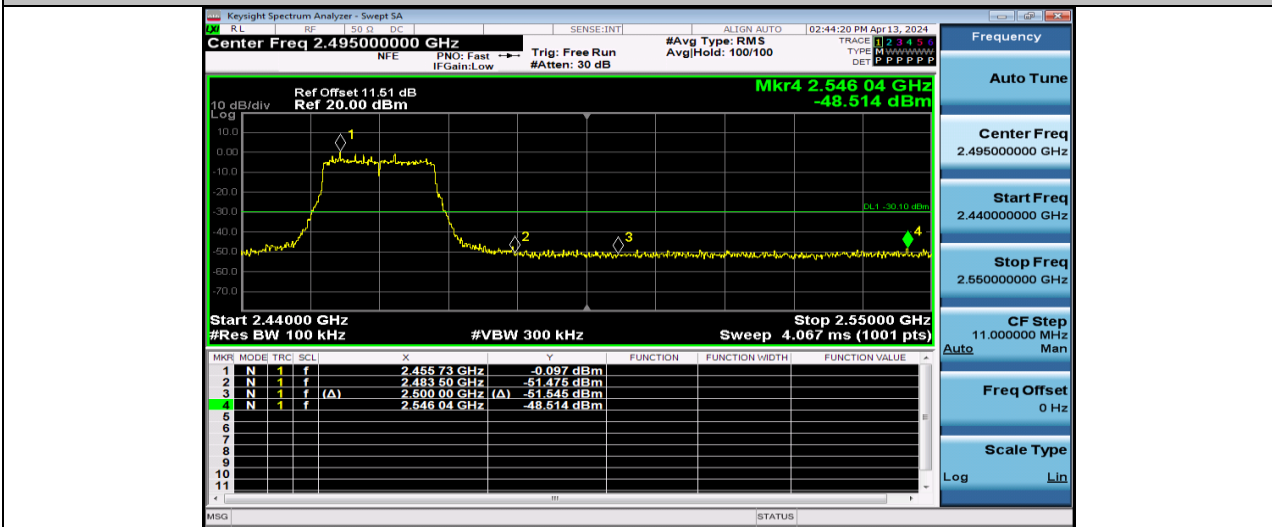
11N20SISO-Ant1-2462-PASS
