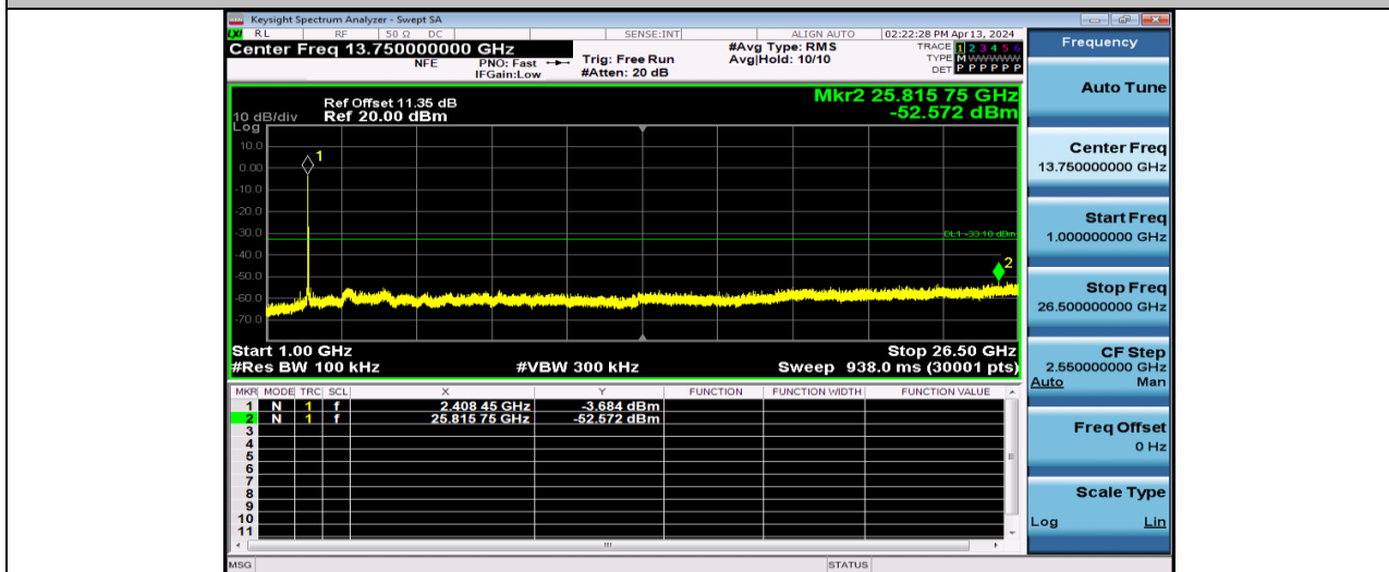
11G-Ant1-2412-1000~26500-PASS
