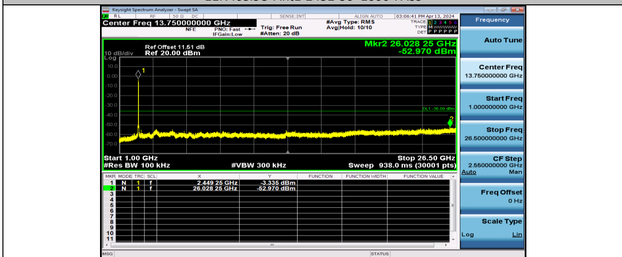
11N40SISO-Ant1-2452-1000~26500-PASS
