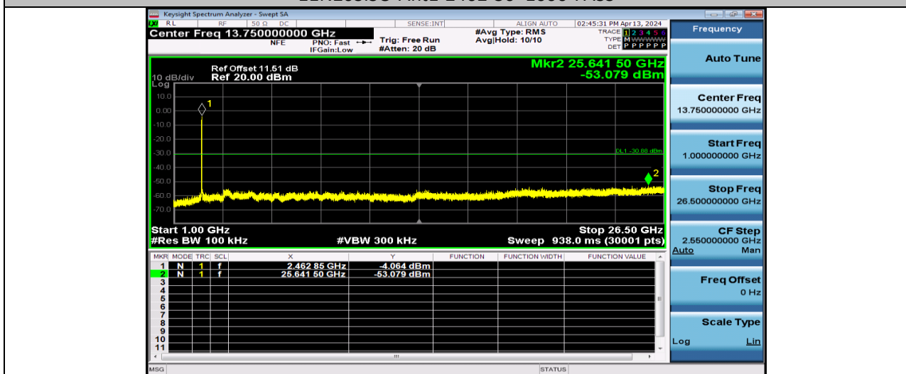
11N20SISO-Ant1-2462-1000~26500-PASS
