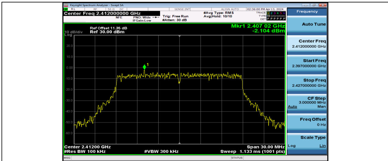
11N20SISO-Ant1-2412-0~Reference-PASS
