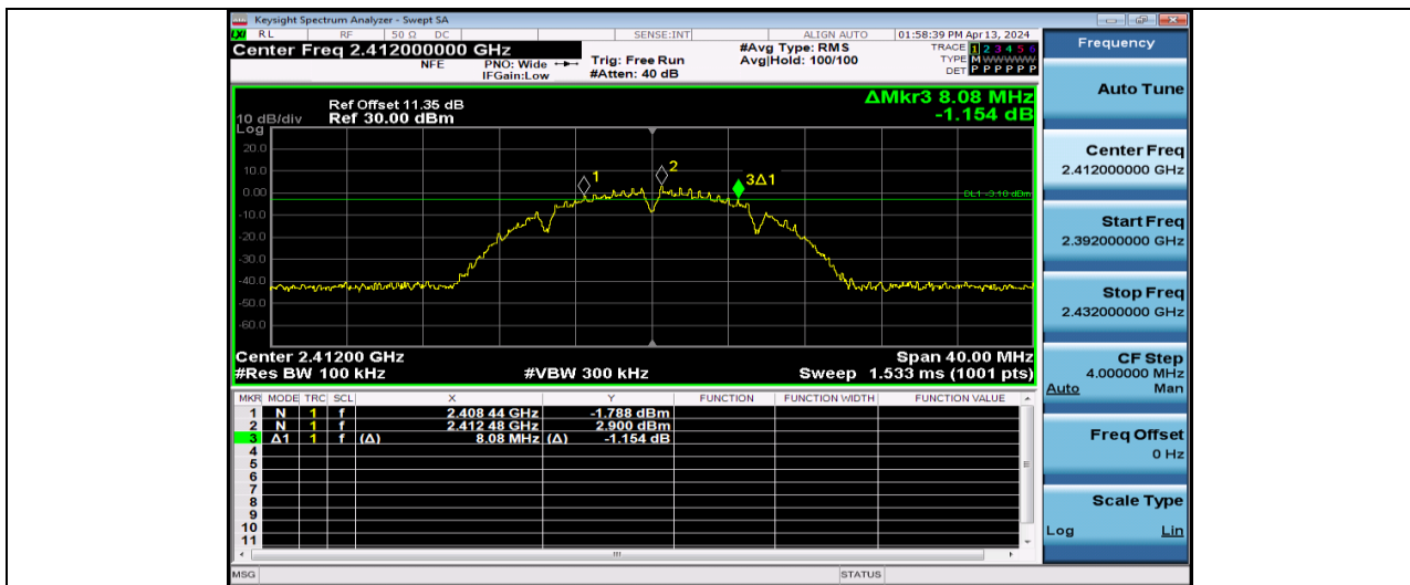
11B-Ant1-2412-PASS
