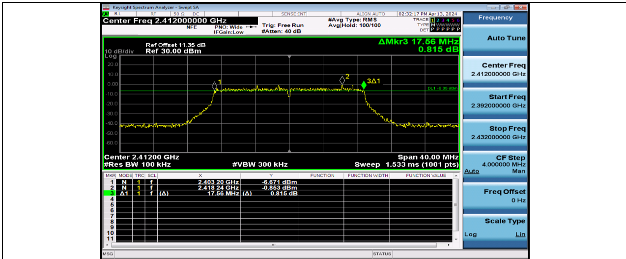
11N20SISO-Ant1-2412-PASS
