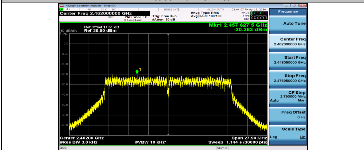
11N20SISO-Ant1-2462-PASS
