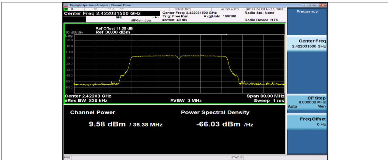
11N40SISO-Ant1-2422-PASS
