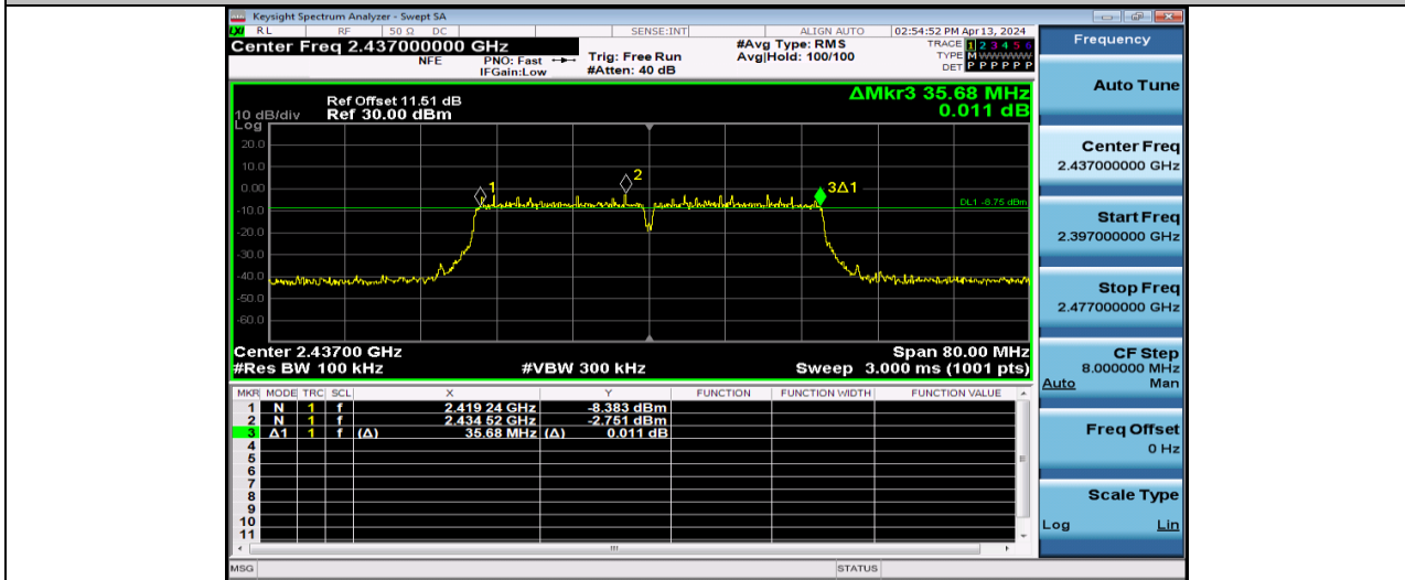
11N40SISO-Ant1-2437-PASS
