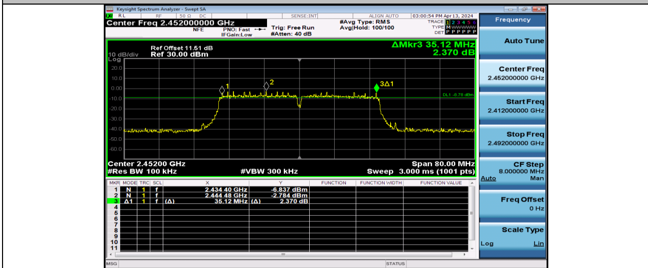
11N40SISO-Ant1-2452-PASS
