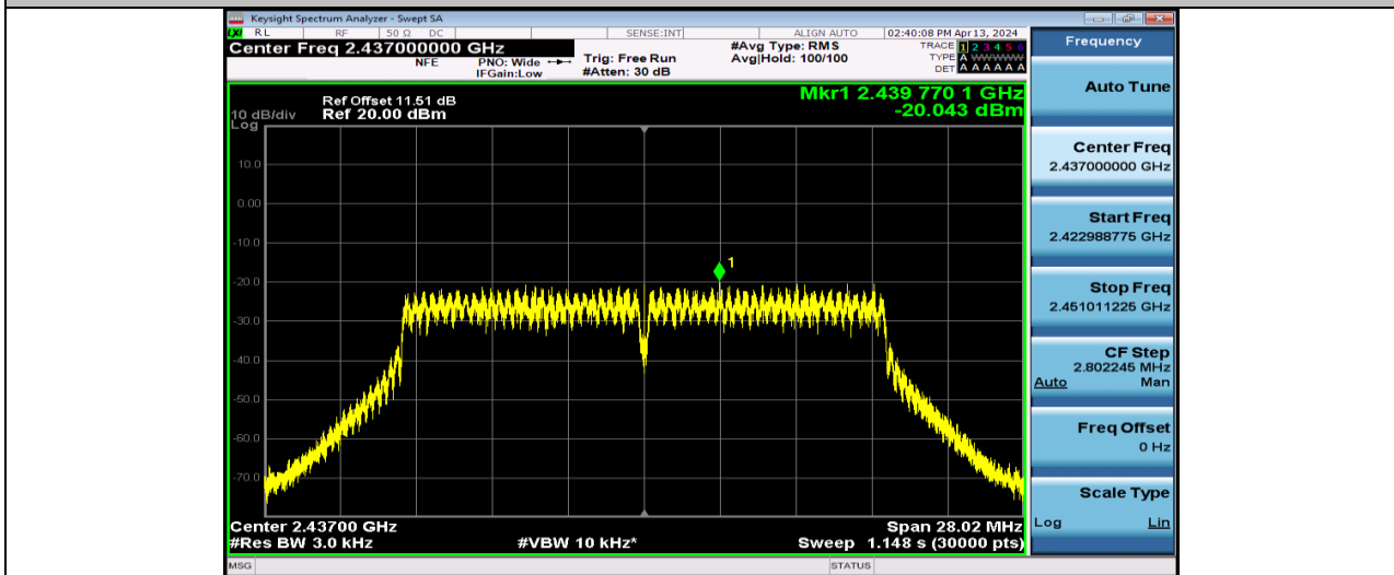
11N20SISO-Ant1-2437-PASS
