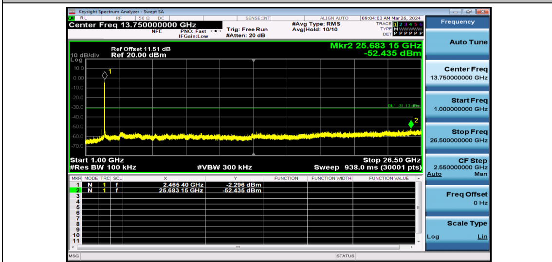
11G-Ant1-2462-1000~26500-PASS
