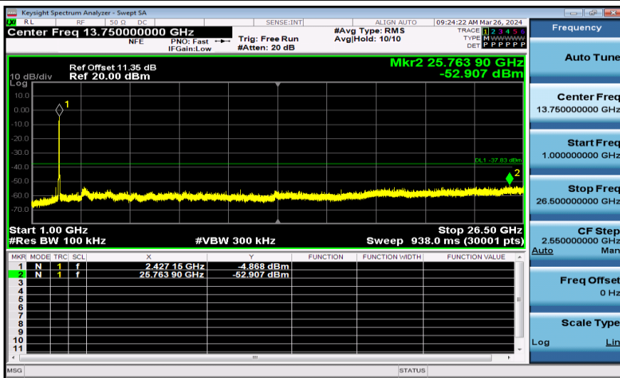
11N40SISO-Ant1-2422-1000~26500-PASS
