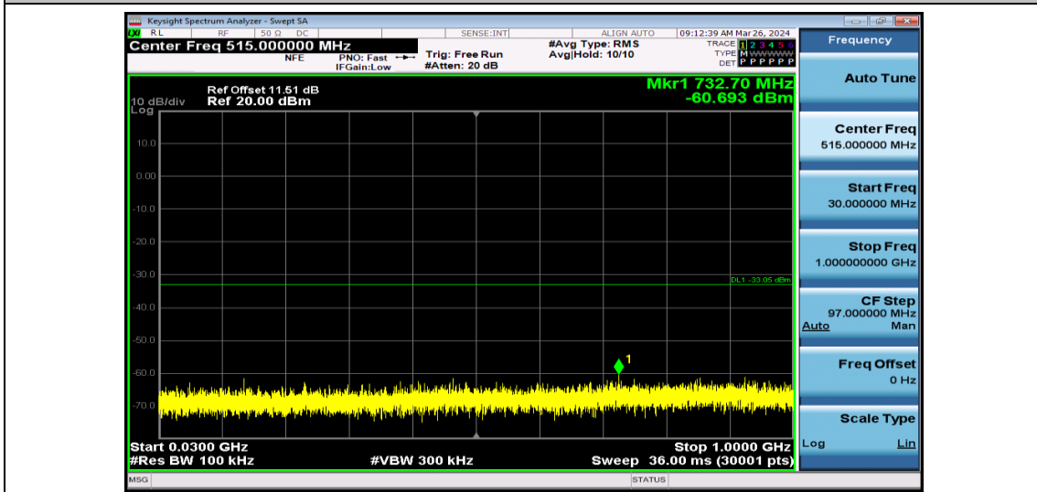
11N20SISO-Ant1-2437-30~1000-PASS
