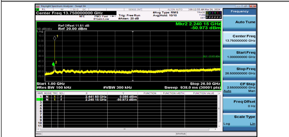
11N20SISO-Ant1-2437-1000~26500-PASS
