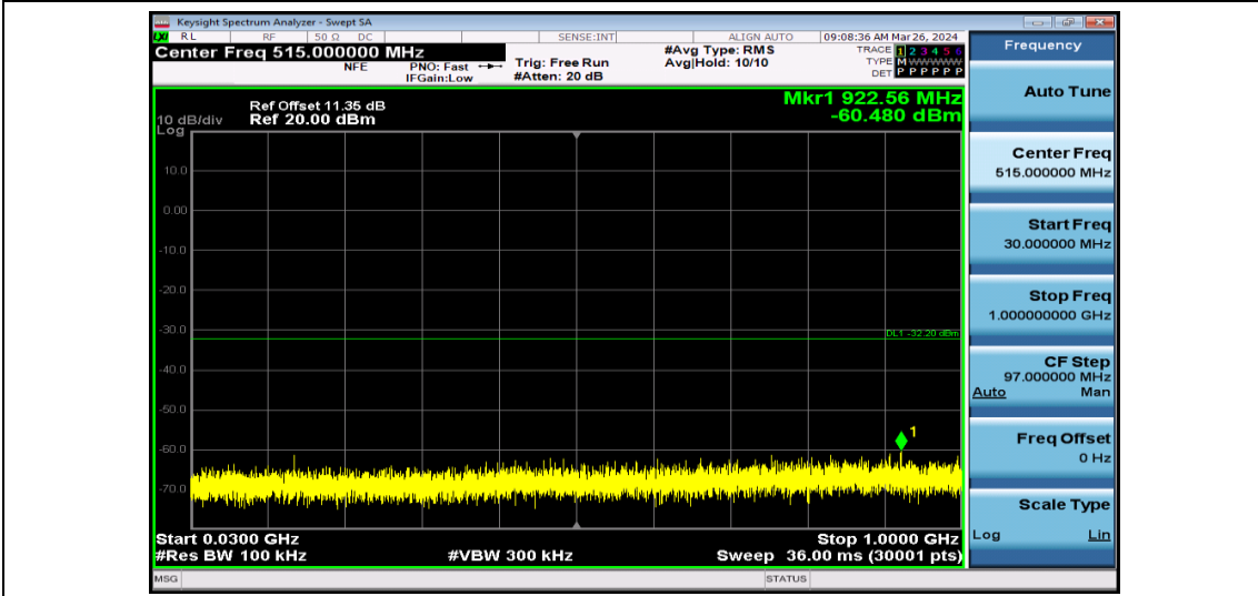
11N20SISO-Ant1-2412-30~1000-PASS
