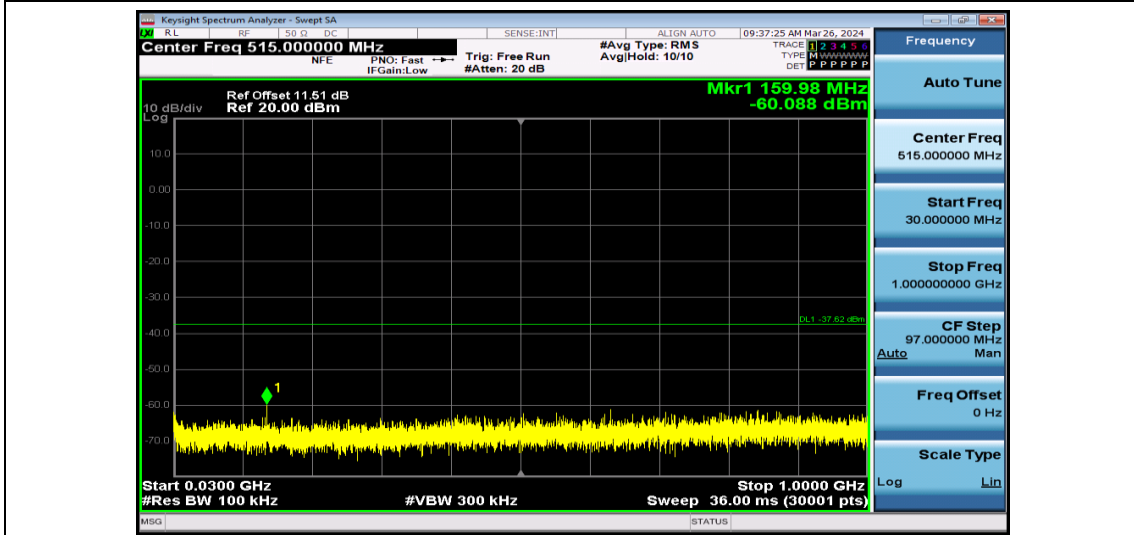
11N40SISO-Ant1-2452-30~1000-PASS
