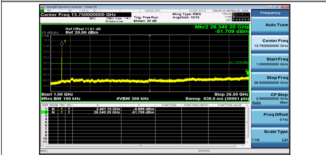
11B-Ant1-2462-1000~26500-PASS
