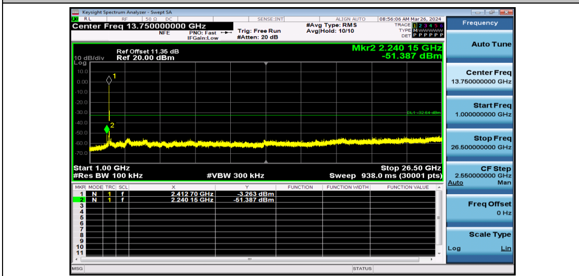
11G-Ant1-2412-1000~26500-PASS
