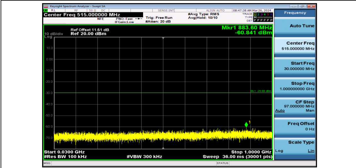
11B-Ant1-2437-30~1000-PASS
