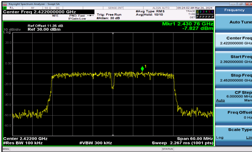
11N40SISO-Ant1-2422-0~Reference-PASS
