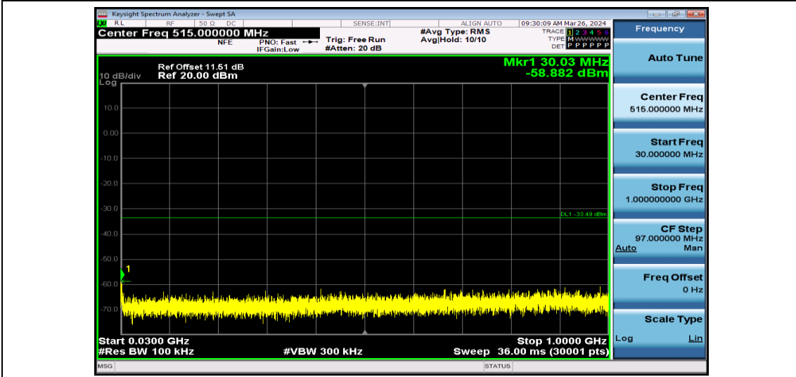
11N40SISO-Ant1-2437-30~1000-PASS
