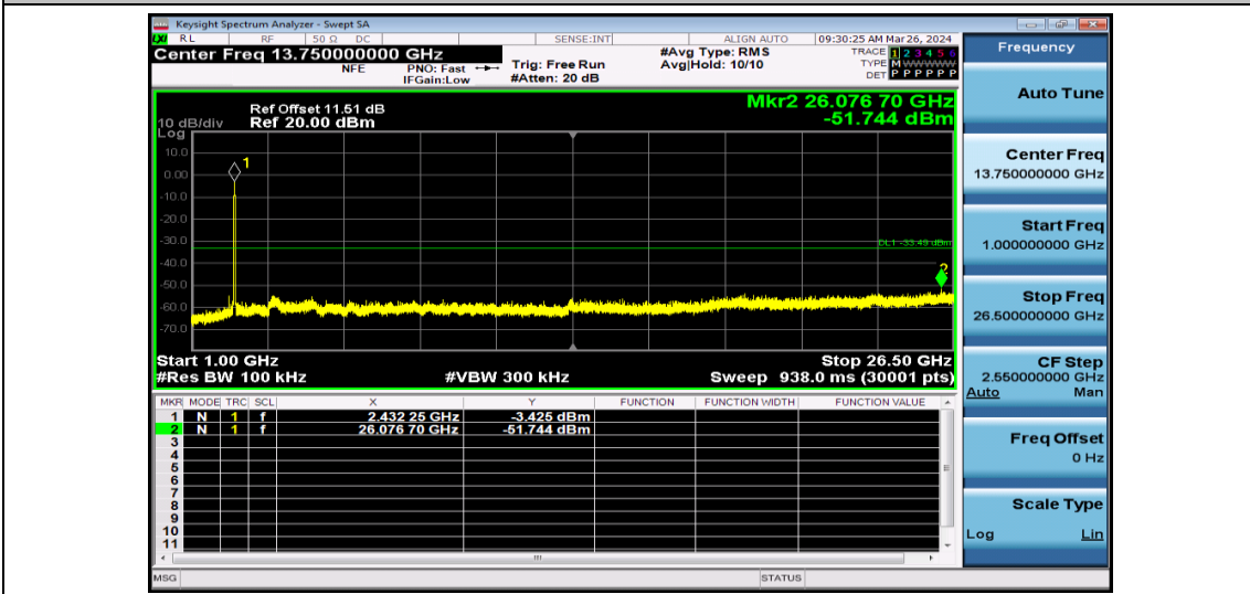
11N40SISO-Ant1-2437-1000~26500-PASS
