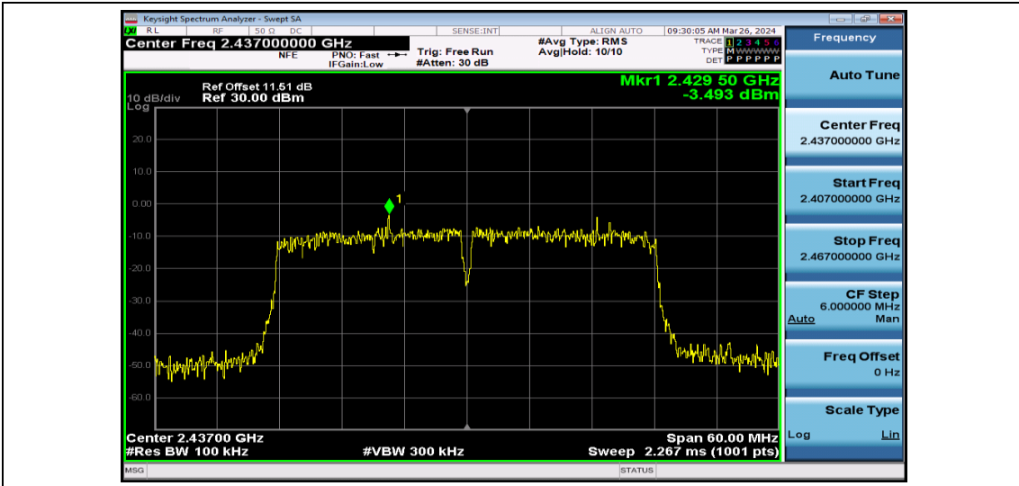
11N40SISO-Ant1-2437-0~Reference-PASS
