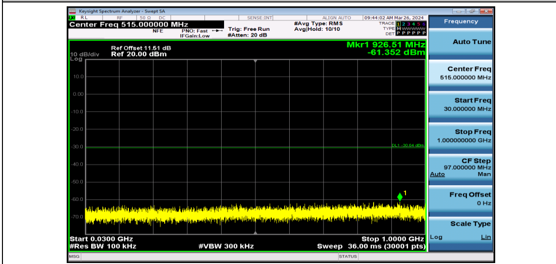
11B-Ant1-2462-30~1000-PASS
