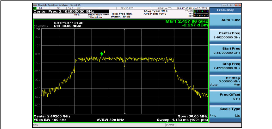
11N20SISO-Ant1-2462-0~Reference-PASS
