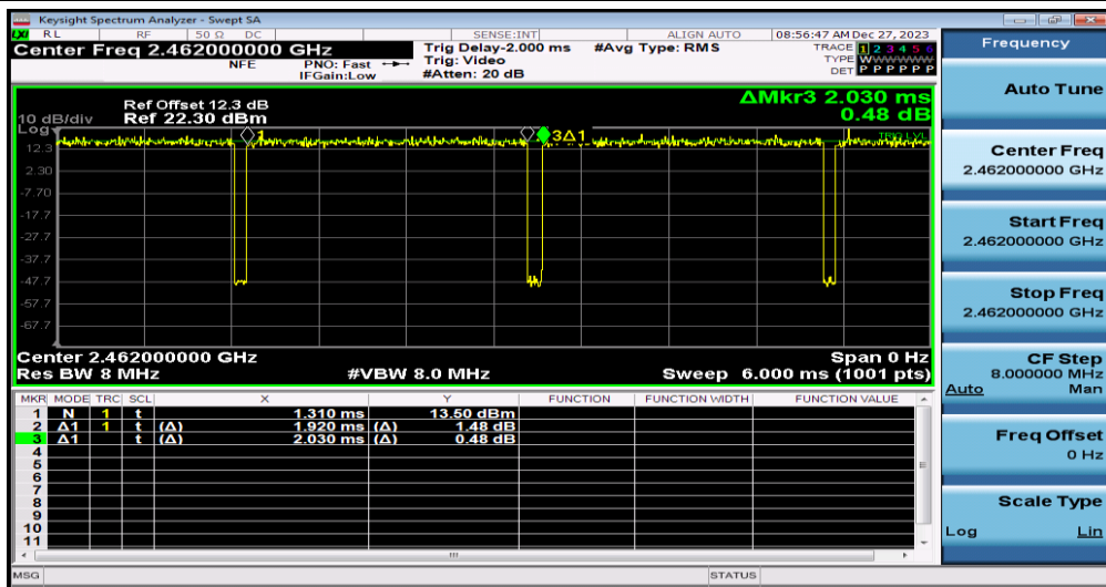
NTNV-11N20SISO-Ant1-2462
