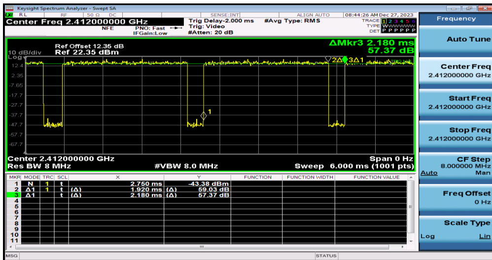
NTNV-11N20SISO-Ant1-2412
