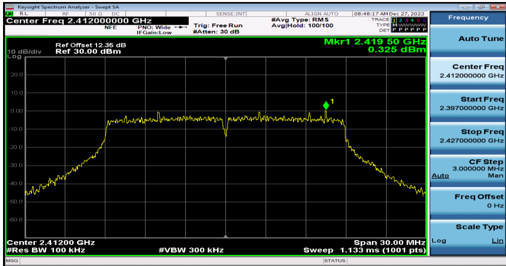
11N20SISO-Ant1-2412-0~Reference
