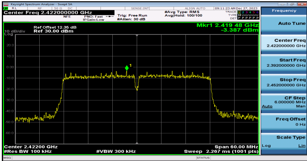
11N40SISO-Ant1-2422-0~Reference
