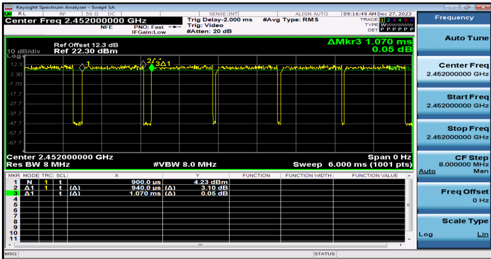
NTNV-11N40SISO-Ant1-2452
