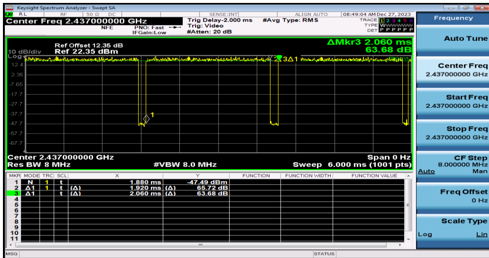
NTNV-11N20SISO-Ant1-2437
