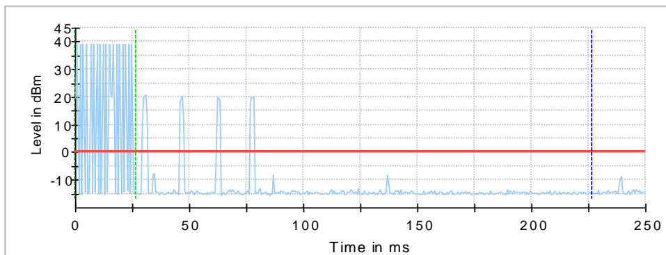
— In-Service Monitoring Channel Move Time first 200ms — Threshold - - - Start of Radar - - - Trigger at end of Radar - - - First 200ms of Channel Closing Tx Time
