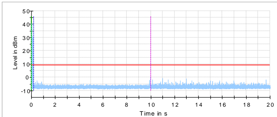
— In-Service Monitoring Channel Move Time Threshold - - - Start of Radar - - - Trigger at end of Radar - - - First 200ms of Channel Closing Tx Time - - - 10sec Channel Move Time Limit
