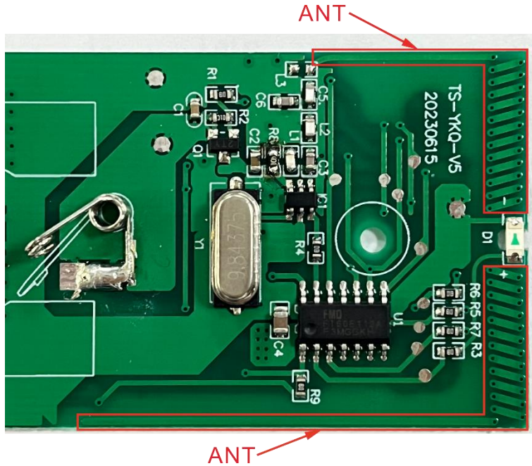
Size of antenna: width 0.7MM, length 200MM
