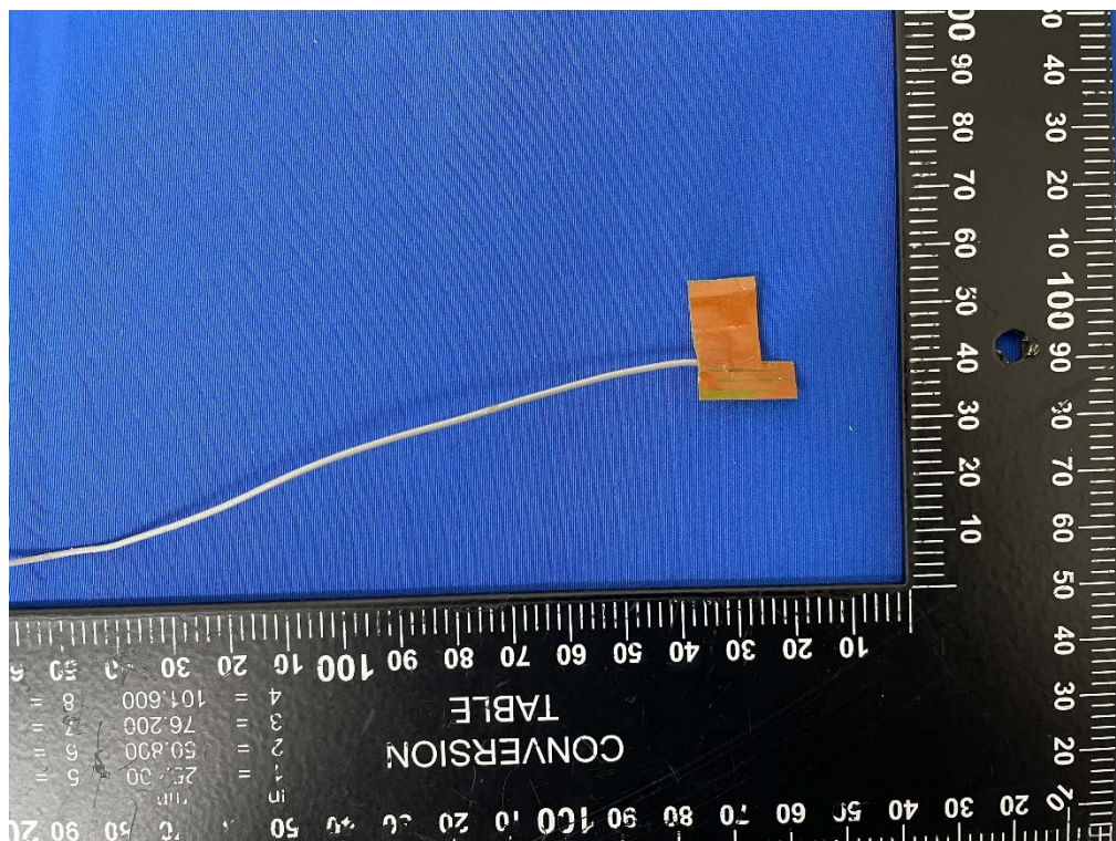
<BT/BLE Antenna>
