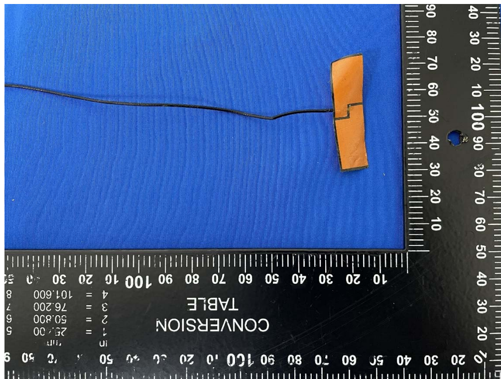
WIFI-Antenna2 (Chain 1)
