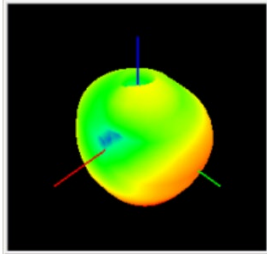
FDD- B17-TRP
