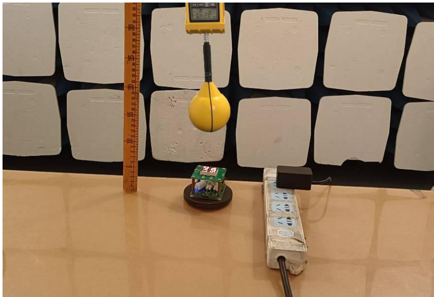
Test Position A - Exposure photo from top surface (TM1) - 15 cm
