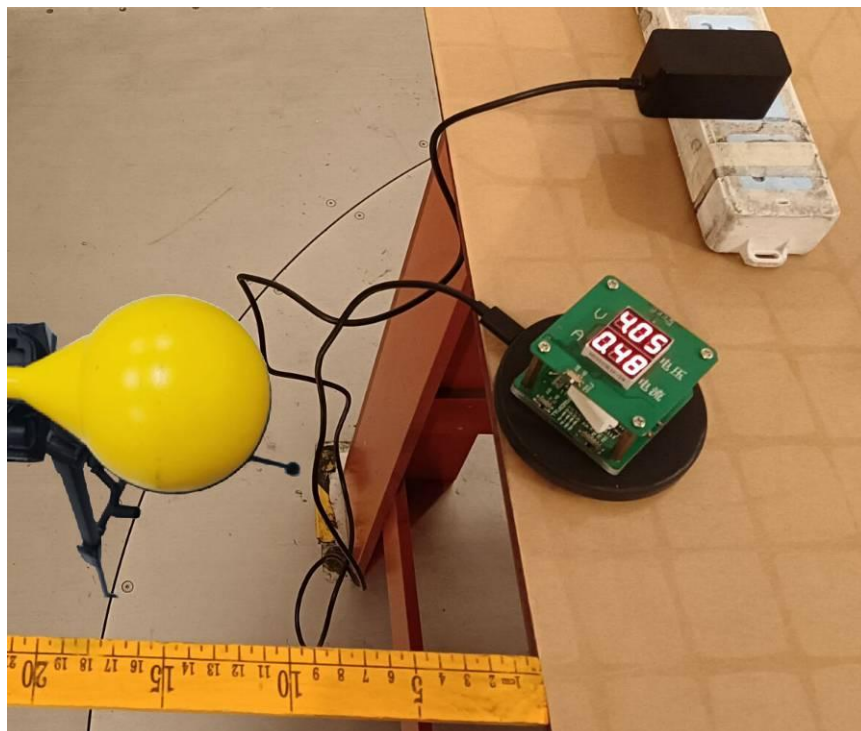
Test Position B - Exposure photo from side edge surface-Rear(TM1) - 15 cm
