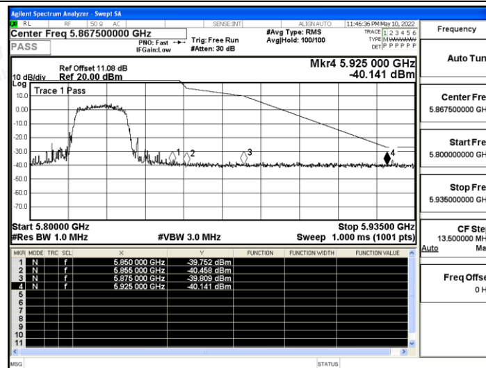
11N20SISO_Ant B_High_5825_Peak
