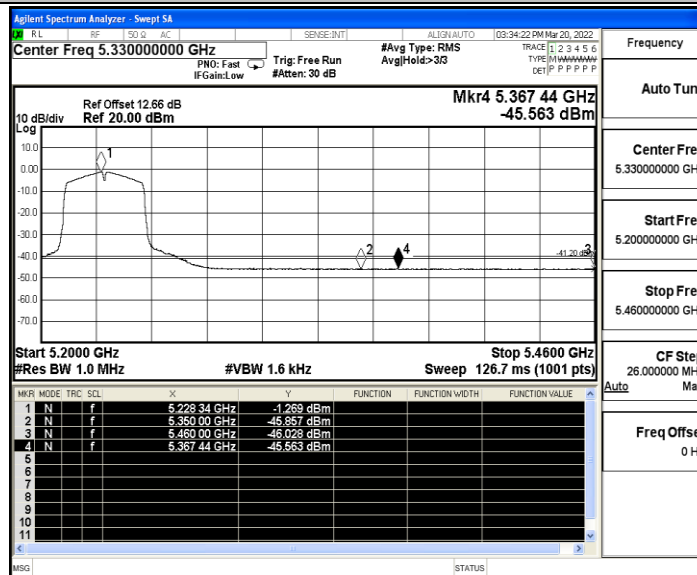
11AC40SISO_MIMO_High_5230_Peak
