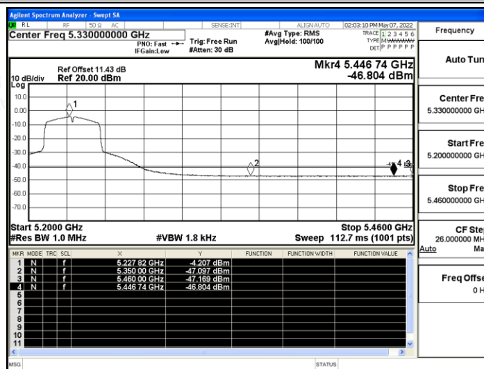
11AX40SISO_Ant A_High_5230_Peak
