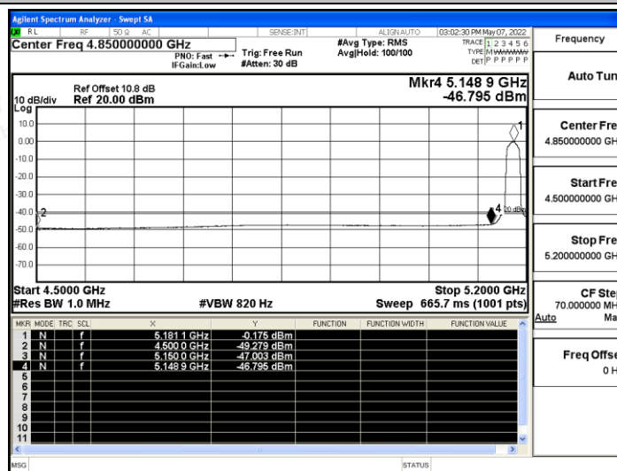
11AC20SISO_Ant A_Low_5180_Peak
