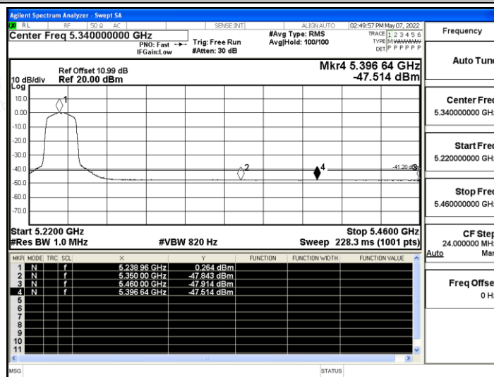
11N20SISO_Ant A_High_5240_Peak
