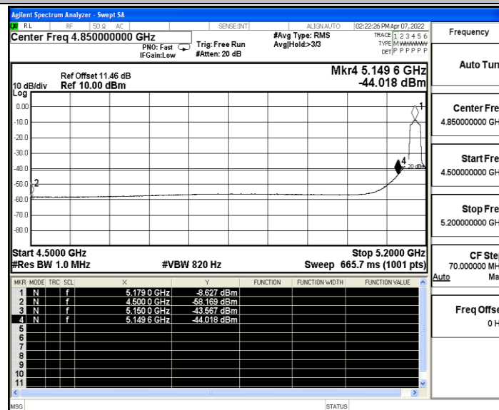
11AX20SISO_MIMO_Low_5180_Peak
