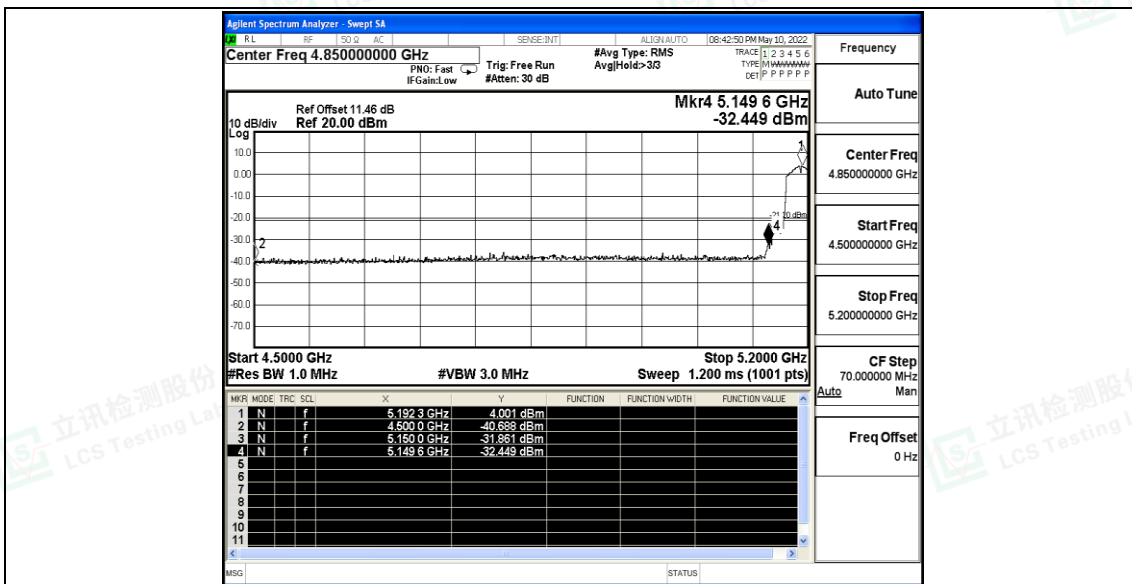
11N40SISO_Ant B_High_5230_AV
