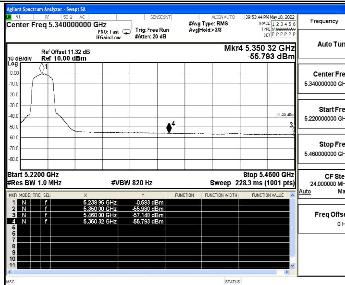
11AX20SISO_Ant B_High_5240_Peak
