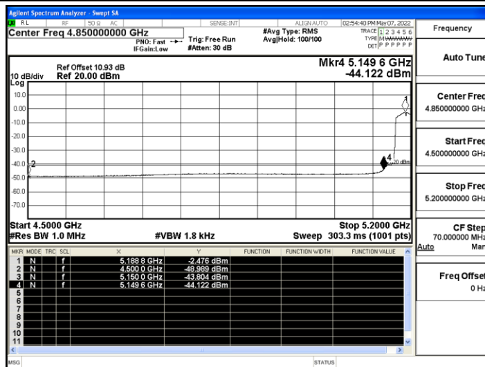
11N40SISO_Ant A_Low_5190_Peak
