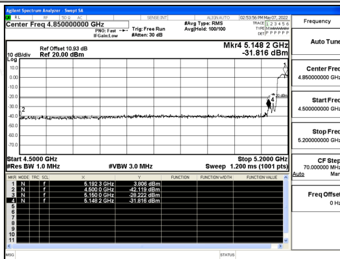
11N40SISO_Ant A_High_5230_AV
