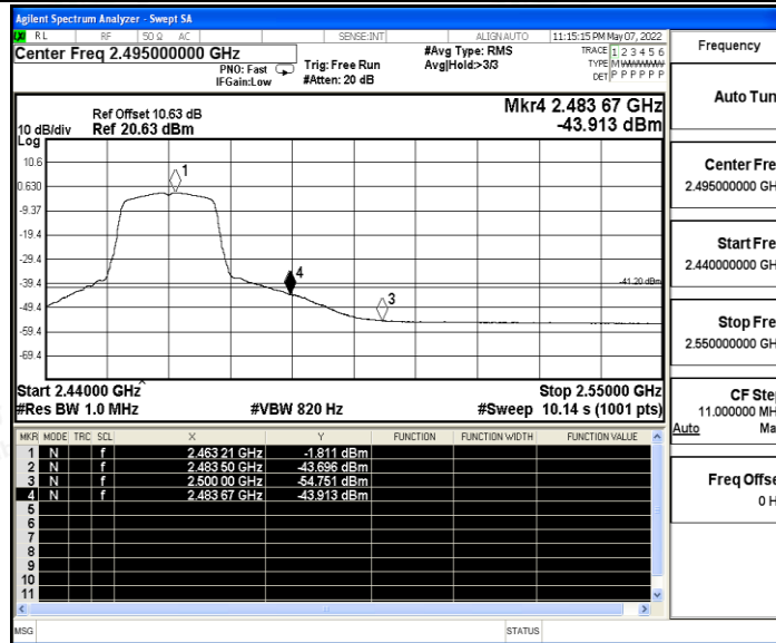
11G_Ant B_High_2462_Peak
