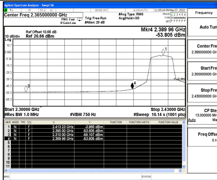
11G_Ant B_Low_2412_Peak
