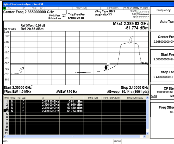
11G_Ant A_Low_2412_Peak
