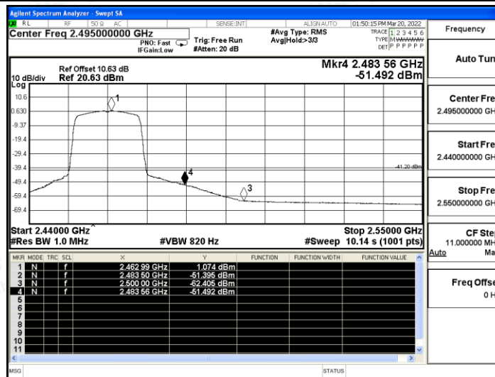
11N20SISO_Ant A_High_2462_Peak
