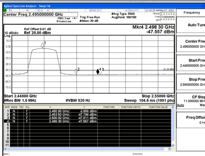
11N20SISO_Ant B_High_2462_Peak
