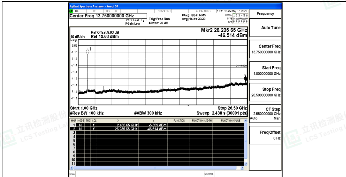
11G_Ant B_2462_0~Reference
