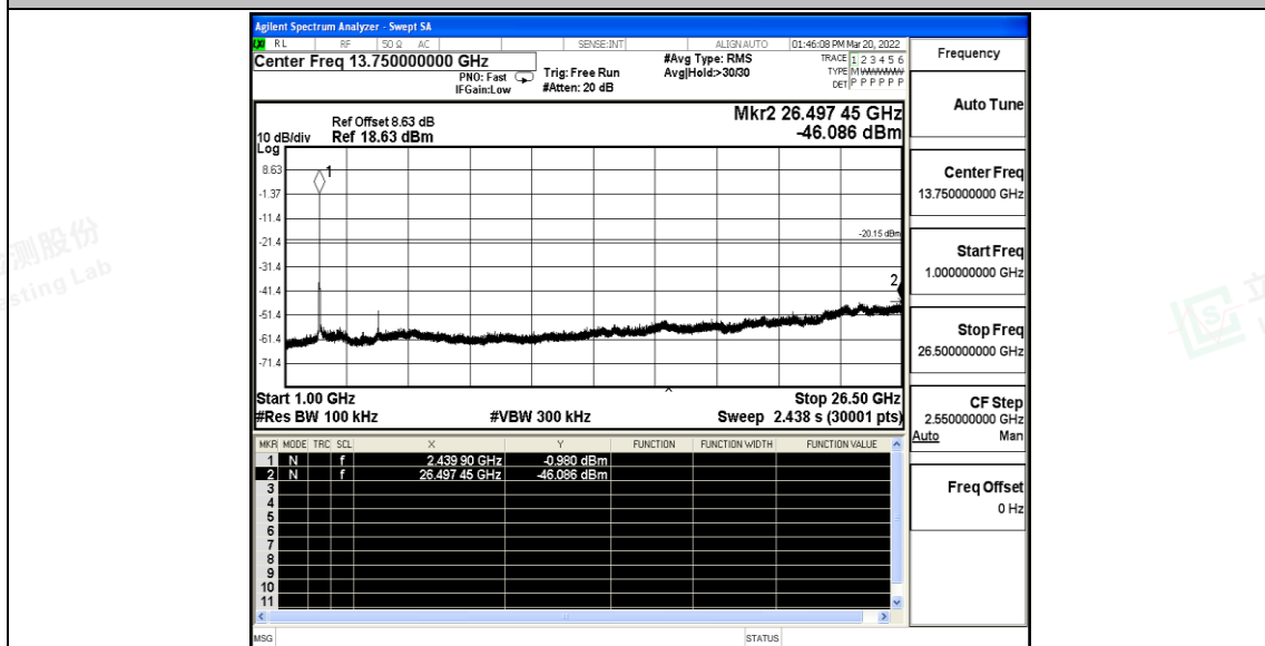
11N20SISO_Ant A_2462_0~Reference
