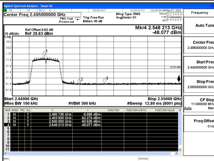
11AX20SISO_Ant B_High_2462
