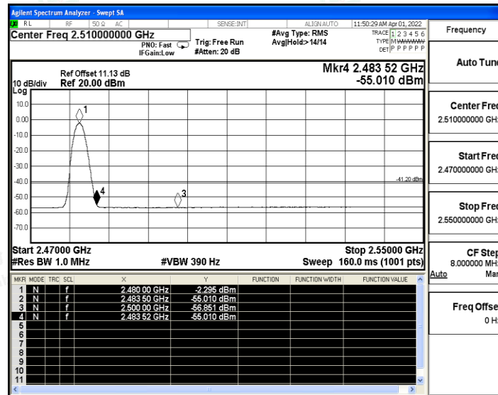
2DH5_Ant1_High_2480_Peak
