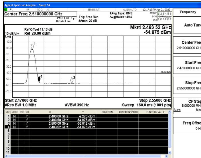
3DH5_Ant1_High_2480_Peak
