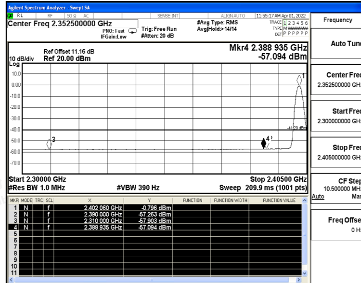
3DH5_Ant1_Low_2402_Peak
