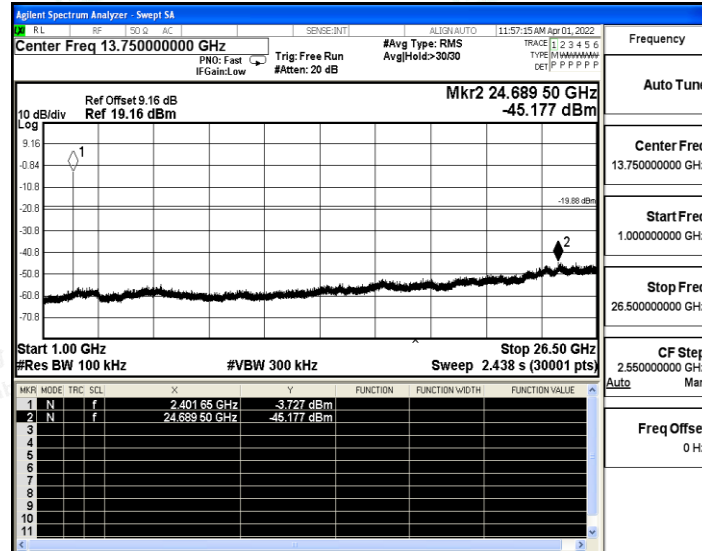
3DH5_Ant1_2441_0~Reference
