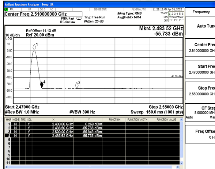
DH5_Ant1_High_2480_Peak
