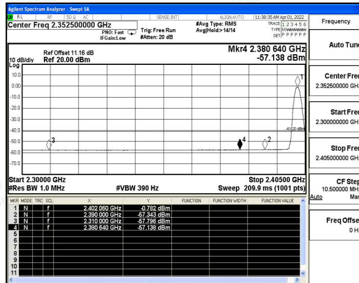
2DH5_Ant1_Low_2402_Peak
