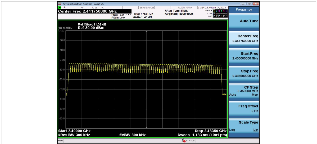
GFSK Modulation
