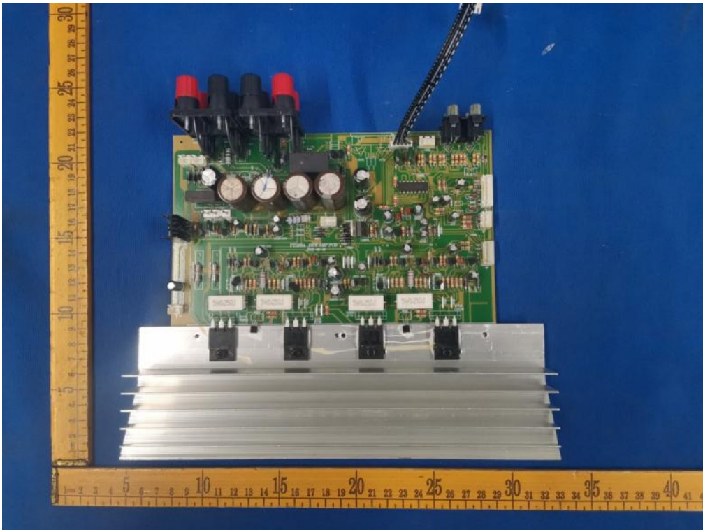
Fig.7(Model: PT260A)
