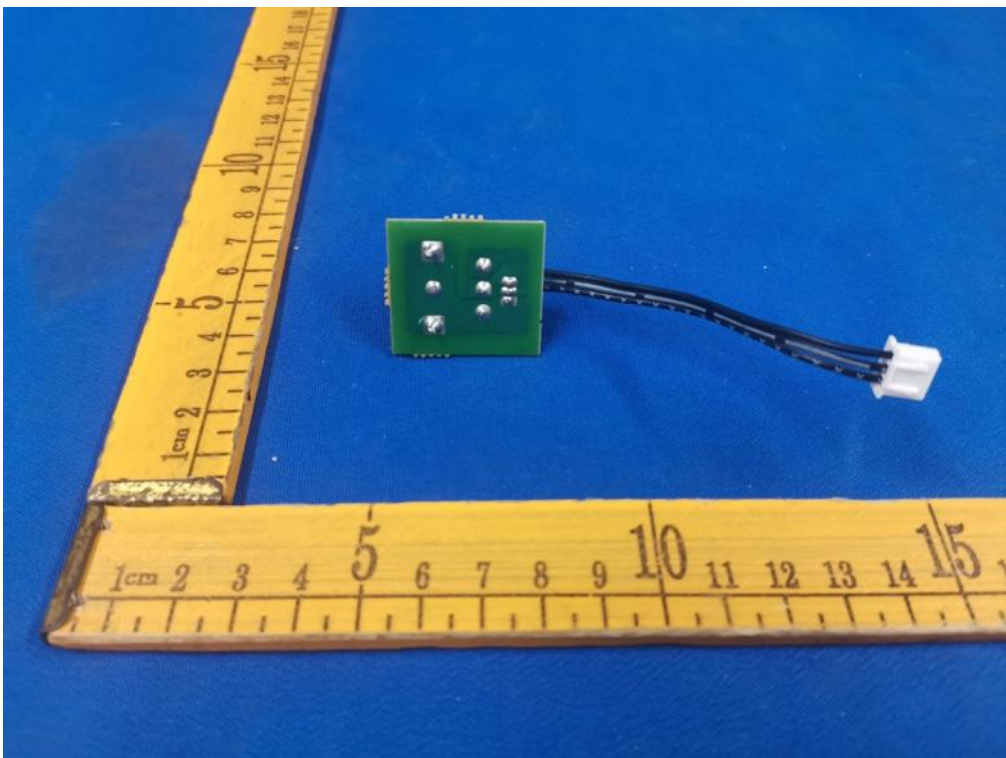
Fig.12(Model: PT260A)
