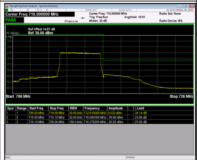
Band17-5MHz-16QAM-23755-1RB#24
