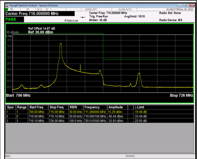
Band17-5MHz-QPSK-23825-25RB#0
