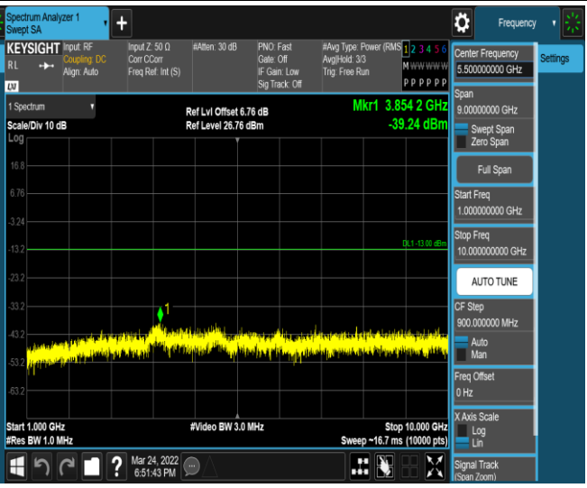
Band12-1.4MHz-QPSK-23095-1RB#0-Range2:1000~10000MHz
