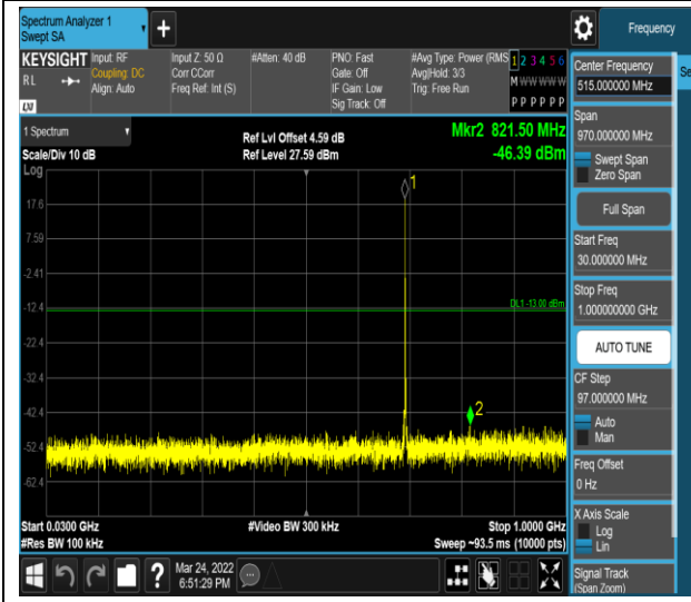
Band12-1.4MHz-QPSK-23095-1RB#0-Range1:30~1000MHz
