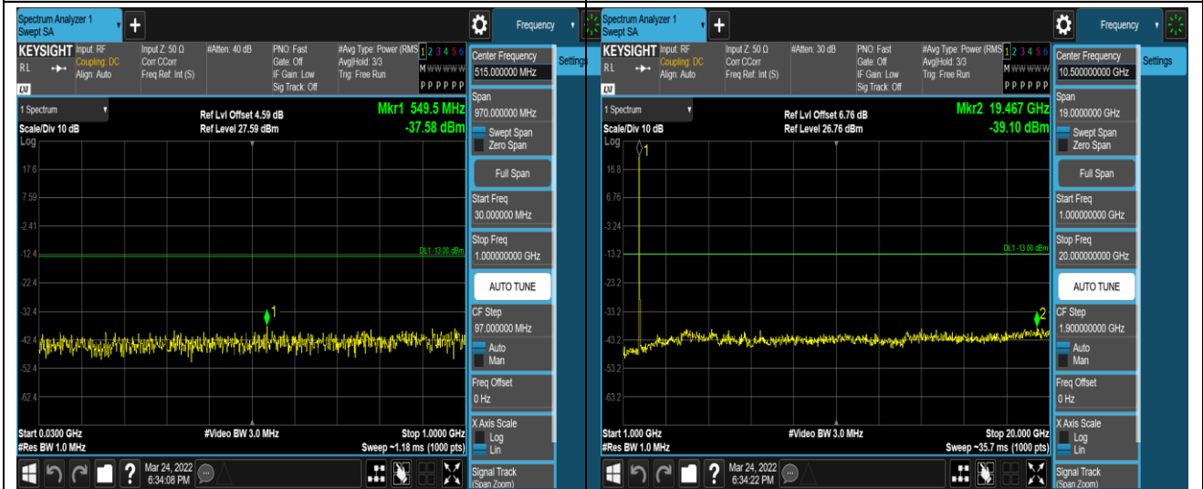
Band4-20MHz-QPSK-20175-1RB#0-Range1:30~1000MHz Band4-20MHz-QPSK-20175-1RB#0-Range2:1000~20000MHz
