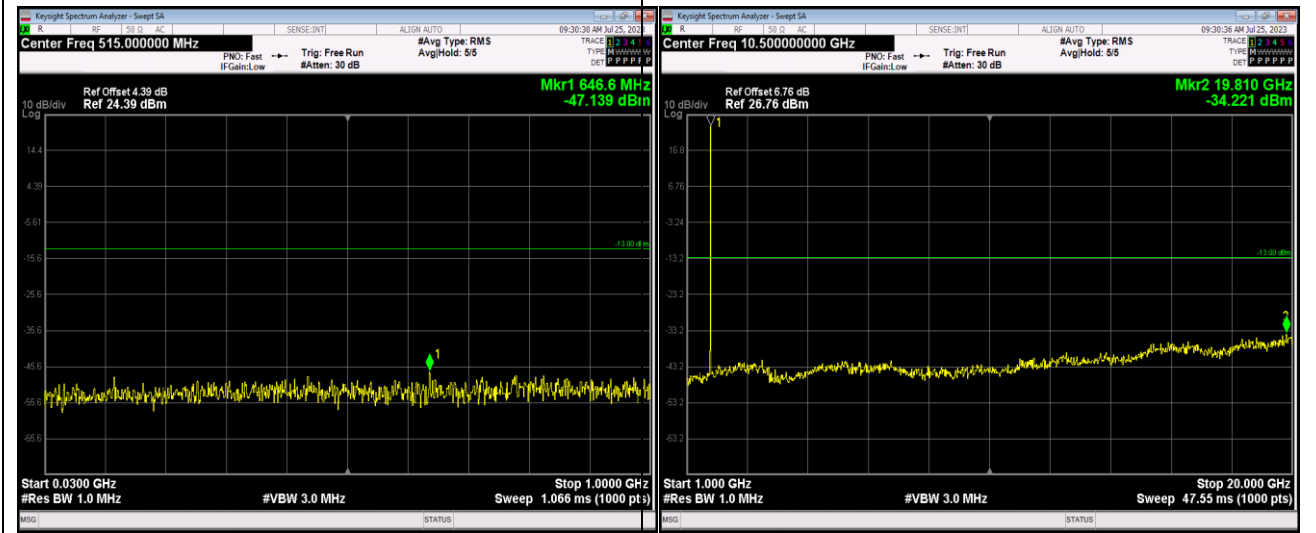
Band4-1.4MHz-64QAM-19957-1RB#0-Range1:30~1000MHz
