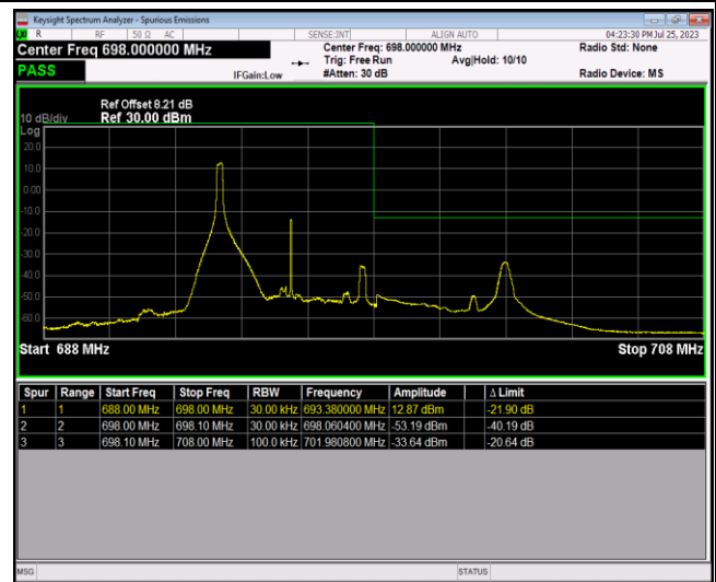
Band71-5MHz-16QAM-133447-25RB#0
