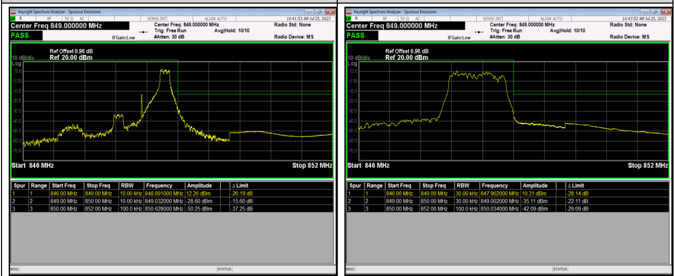
Band5-1.4MHz-64QAM-20407-1RB#0
