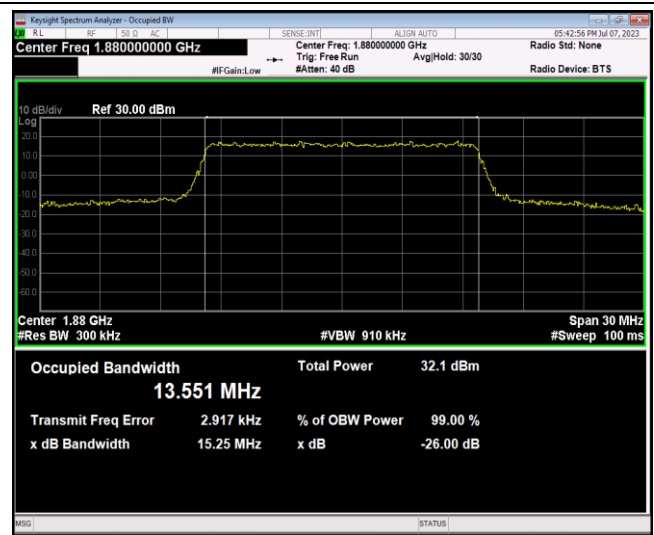
Band2-15MHz-16QAM-18675-75RB#0
