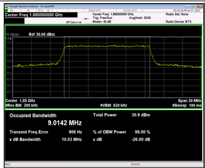
Band2-10MHz-64QAM-18650-50RB#0
