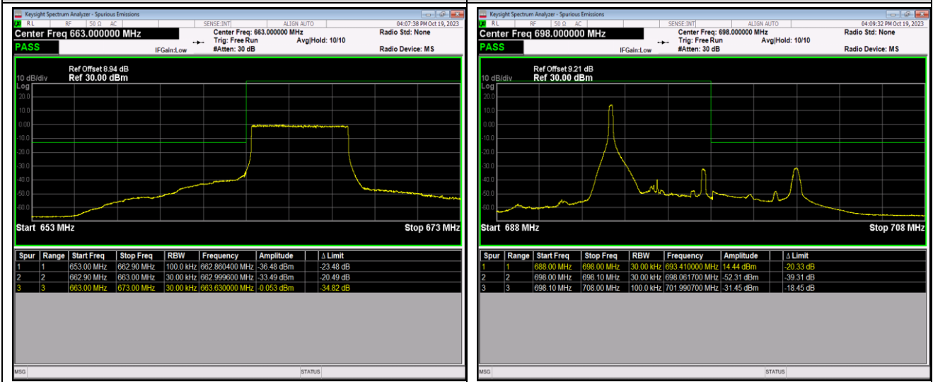
Band71-5MHz-16QAM-133447-1RB#24
