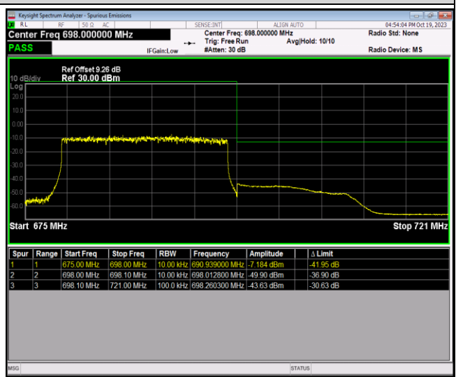
Band71-20MHz-64QAM-133222-1RB#99
