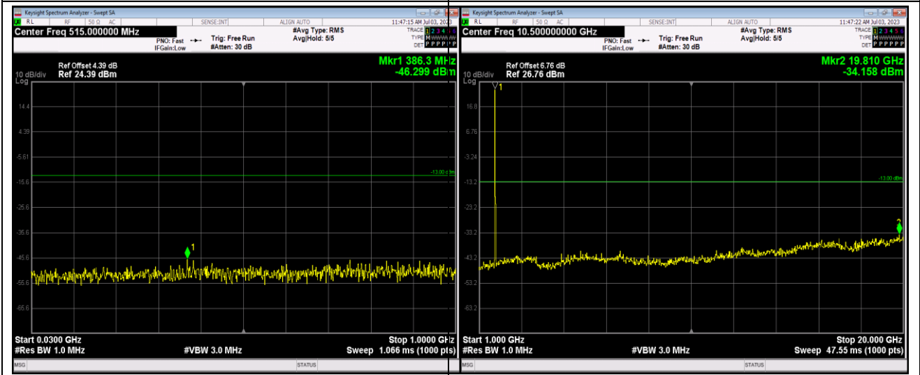
Band4-20MHz-64QAM-20175-1RB#0-Range1:30~1000MHz
