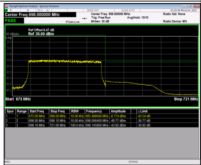
Band71-20MHz-64QAM-133222-1RB#99
