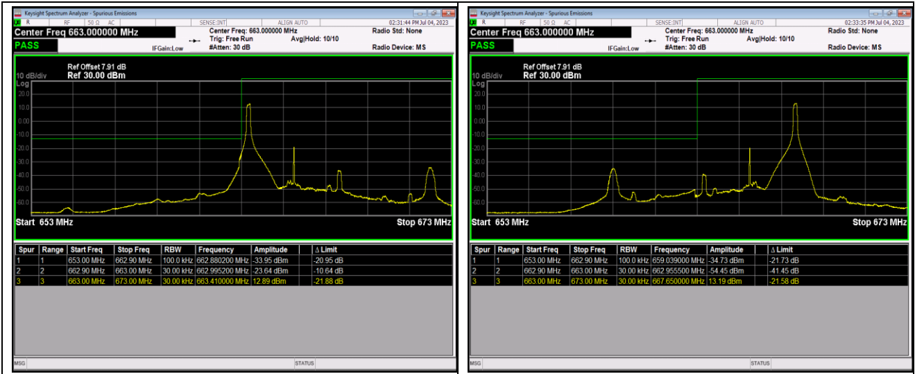
Band71-5MHz-64QAM-133147-25RB#0
