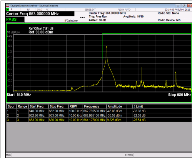
Band71-20MHz-16QAM-133222-100RB#0
