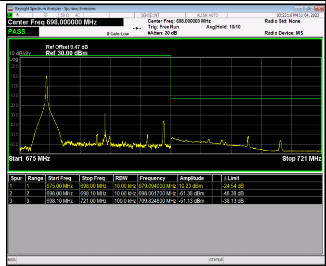
Band71-20MHz-16QAM-133372-100RB#0
