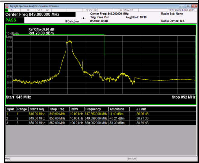
Band5-1.4MHz-64QAM-20643-6RB#0
