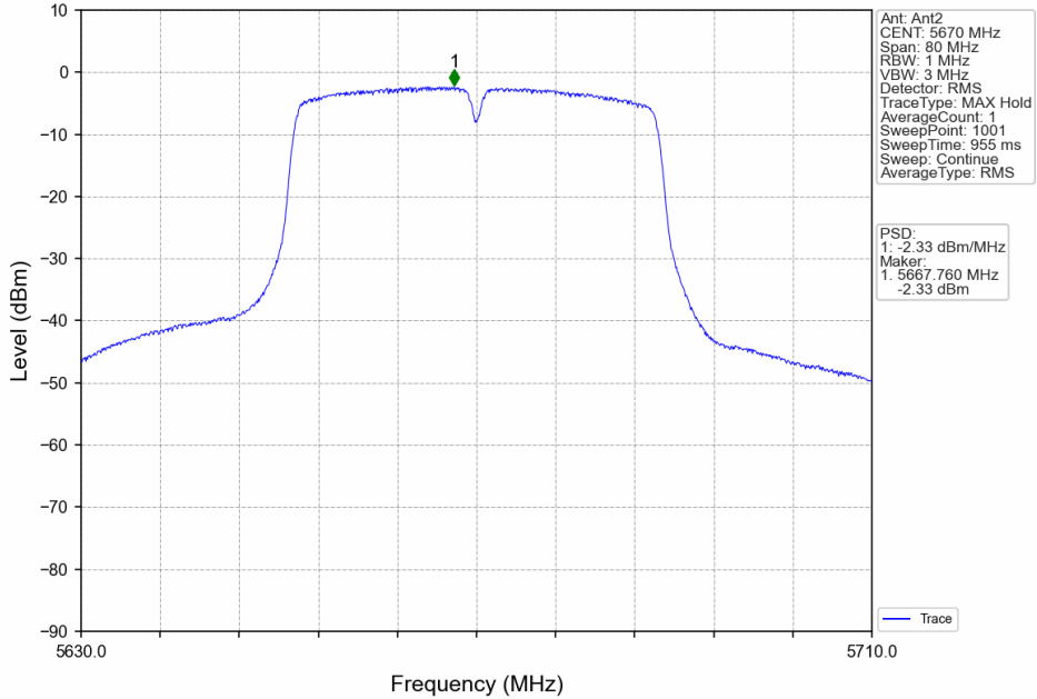
802.11ac(VHT40)_HCH_5670MHz_MIMO_NTNV
