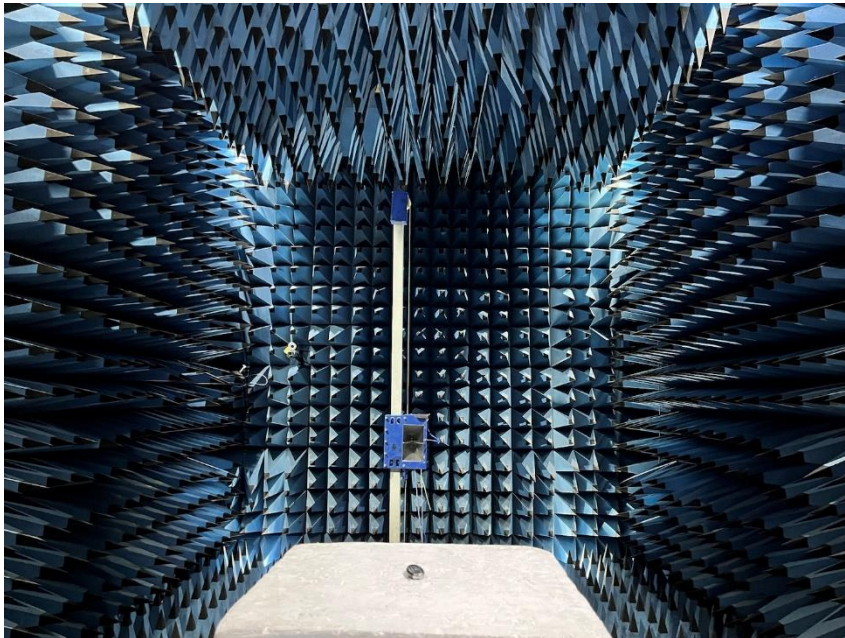
RF Radiated Test (above 1GHz)
