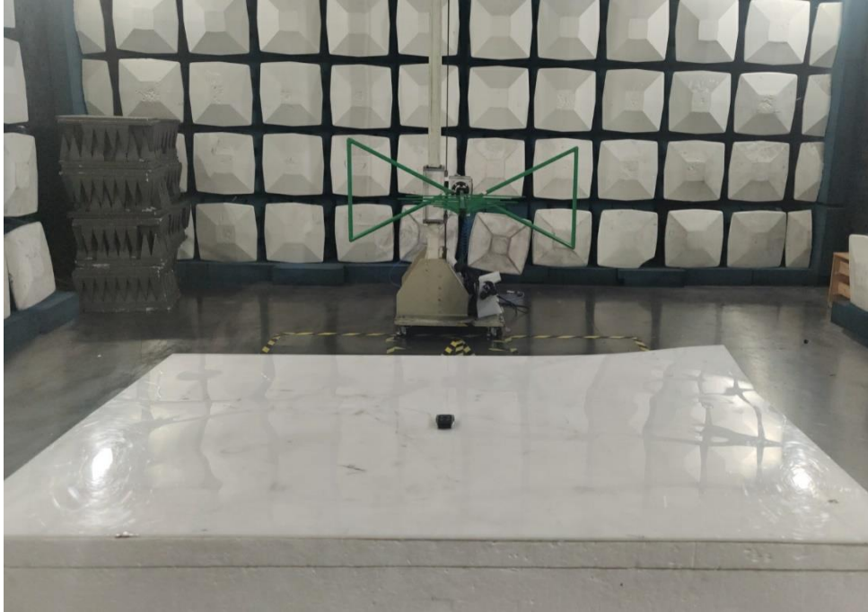
Radiated Emissions below 1GHz
