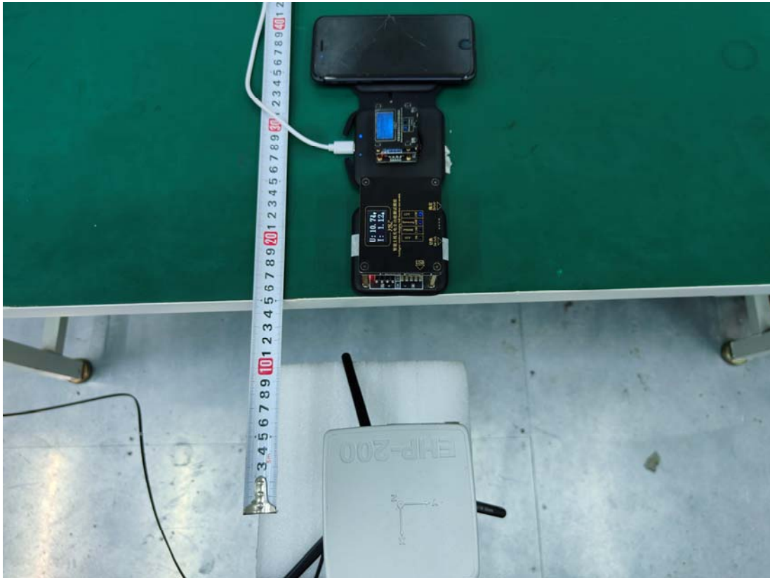
H-Field Position C_M2
