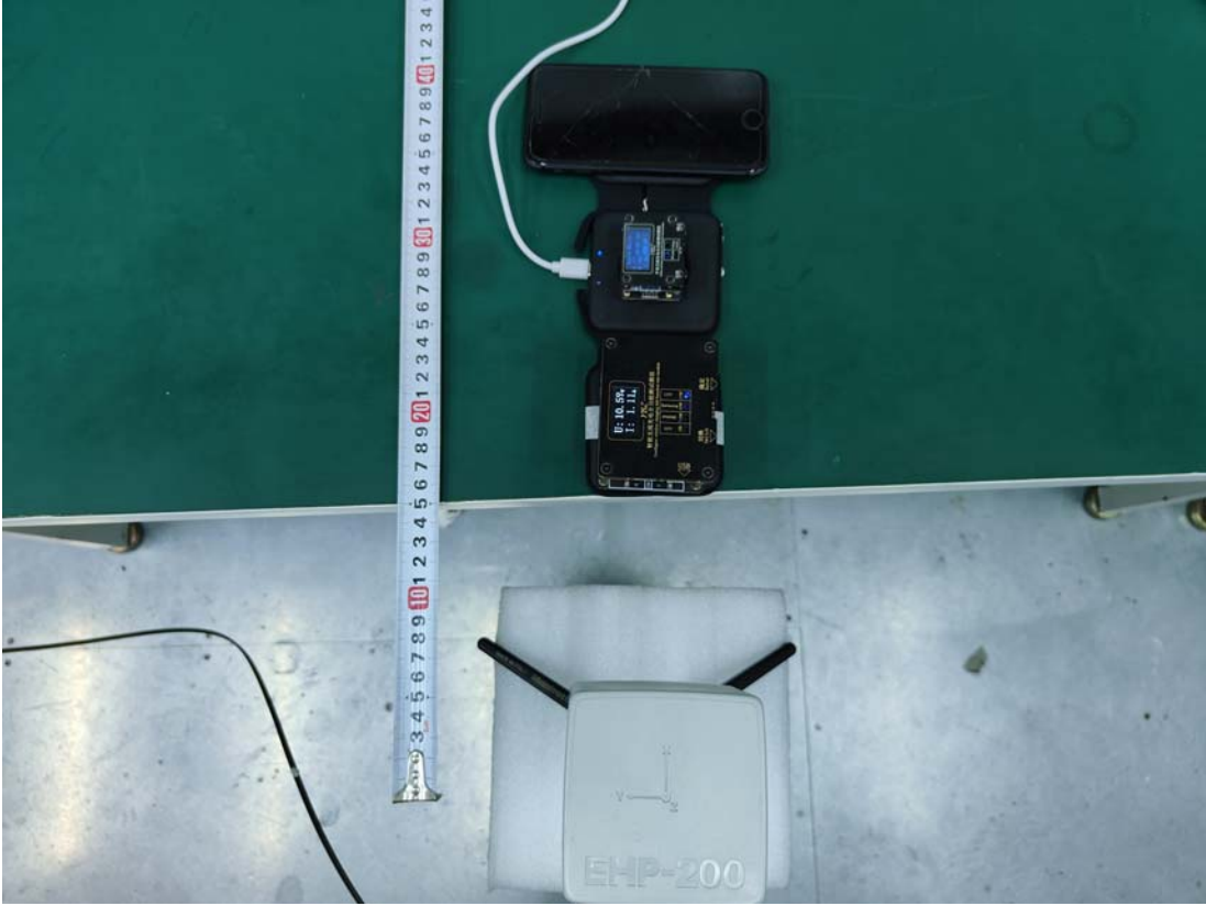
H-Field Position B_M2
